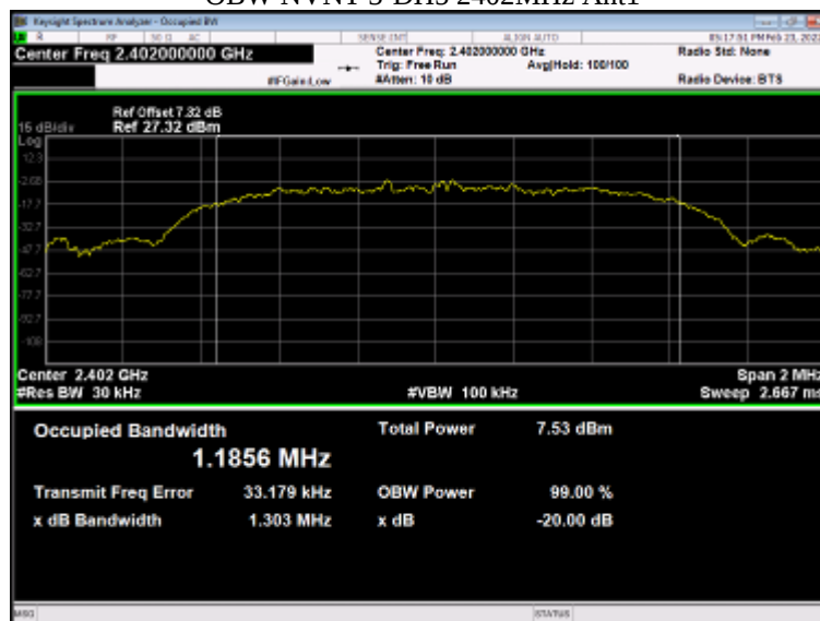
OBW NVNT 3-DH5 2402MHz Ant1
