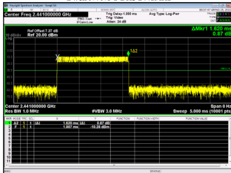
Dwell NVNT 1-DH3 2441MHz
