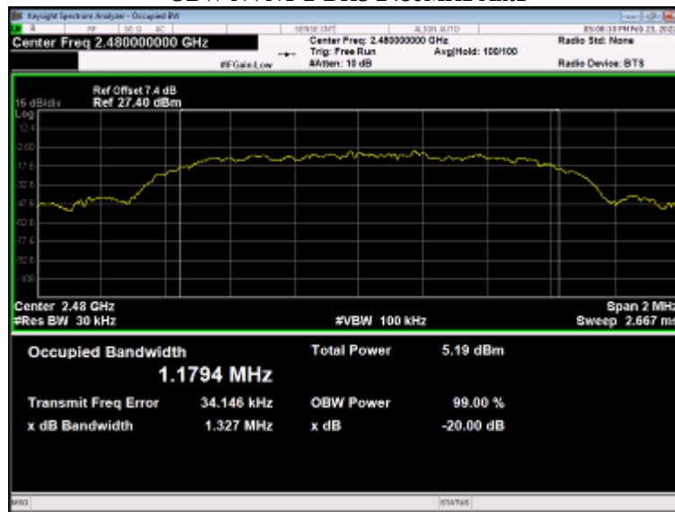
OBW NVNT 2-DH5 2480MHz Ant1
