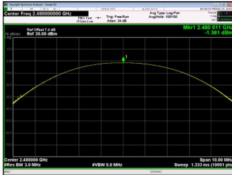
Power NVNT 1-DH5 2480MHz Ant1
