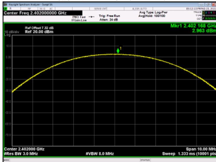
Power NVNT 2-DH5 2402MHz Ant1
