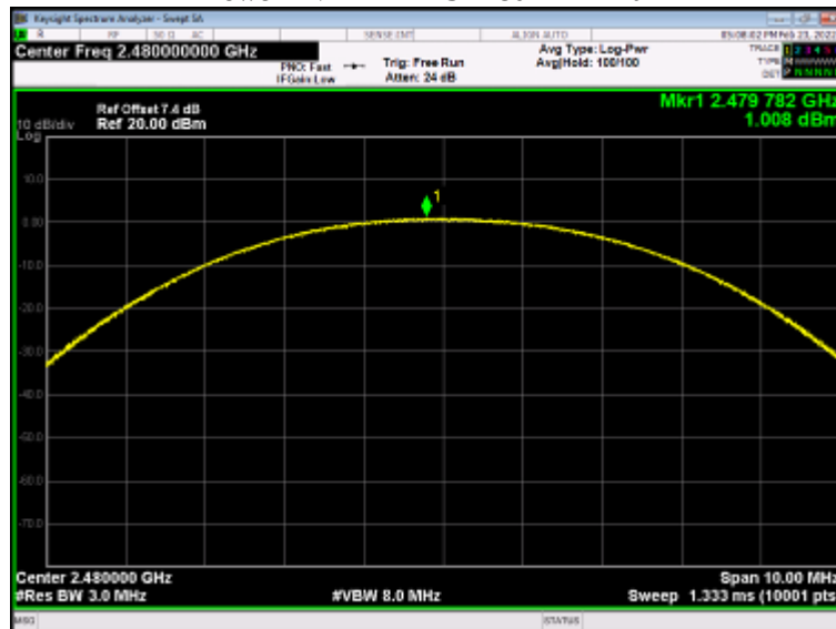
Power NVNT 2-DH5 2480MHz Ant1
