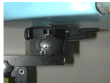
Figure 18. AMPS Body SAR Test Setup w/ Belt Clip
