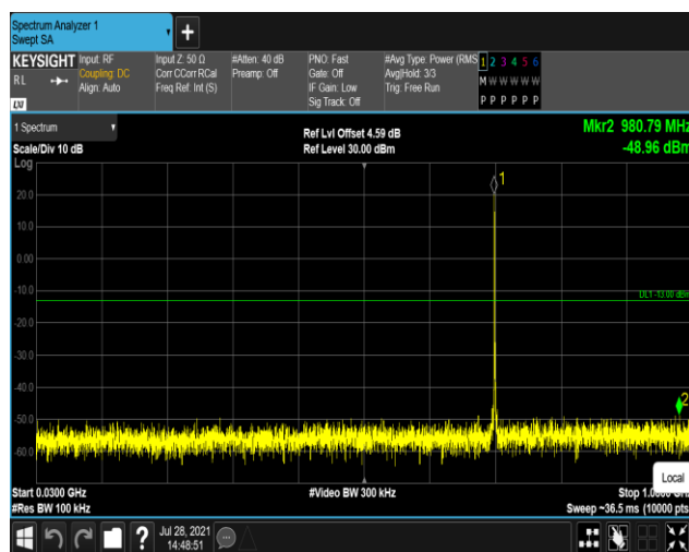
Band12-1.4MHz-QPSK-23173:30~1000MHz
