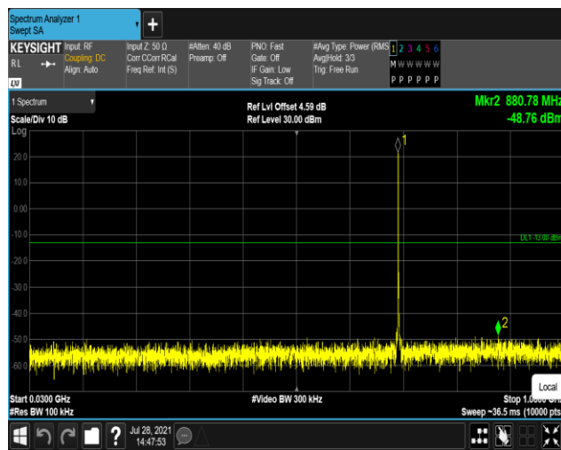
Band12-1.4MHz-16QAM-23095:30~1000MHz
