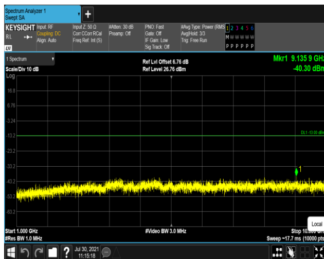
Band13-10MHz-16QAM-23230:1000~10000MHz
