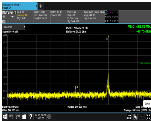
Band12-10MHz-QPSK-23095:30~1000MHz
