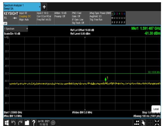
Band13-10MHz-16QAM-23230:1559~1610MHz
