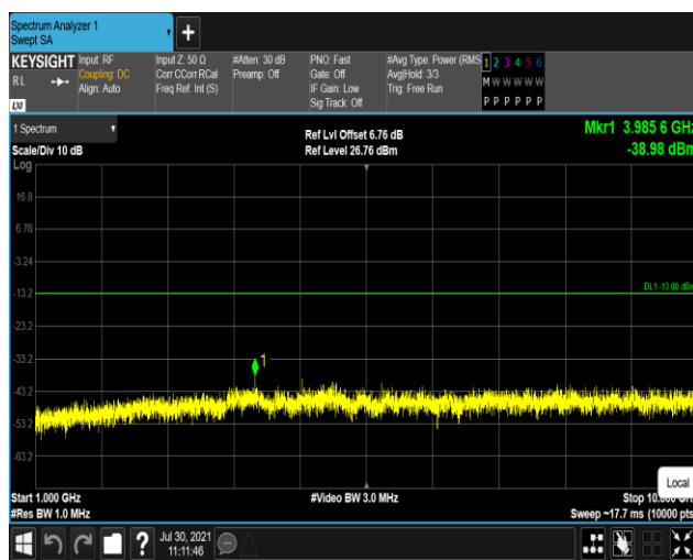
Band13-5MHz-16QAM-23205:1000~10000MHz
