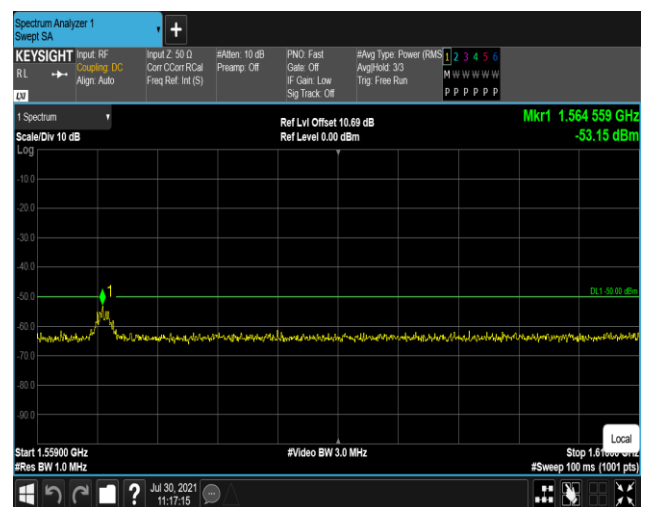
Band13-5MHz-16QAM-23255:1559~1610MHz
