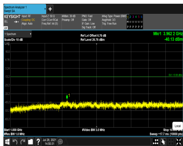
Band12-1.4MHz-QPSK-23173:1000~10000MHz
