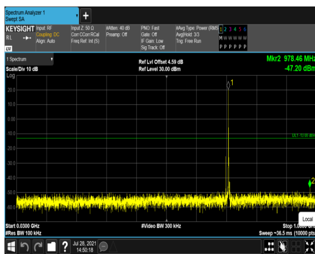
Band12-1.4MHz-QPSK-23173:30~1000MHz
