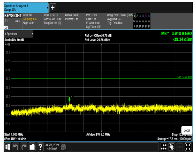
Band12-10MHz-QPSK-23130:1000~10000MHz
