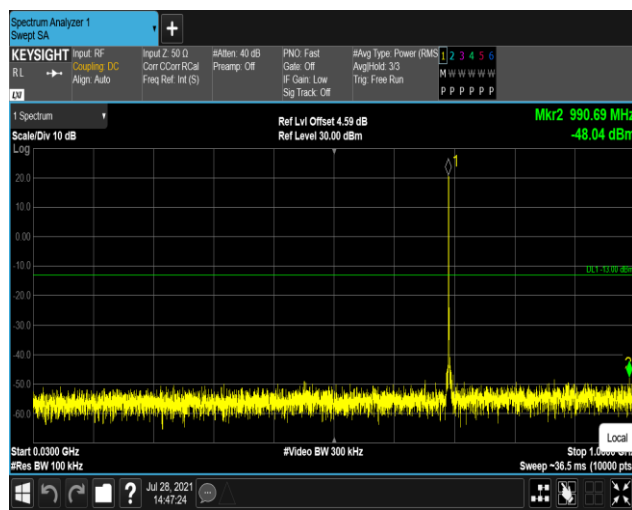
Band12-1.4MHz-QPSK-23095:30~1000MHz
