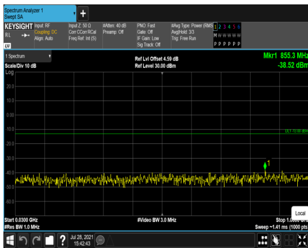
Band25-1.4MHz-QPSK-26365:30~1000MHz
