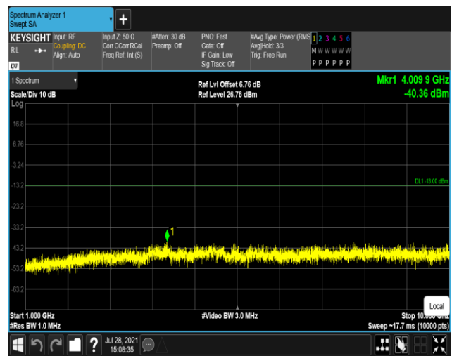
Band12-10MHz-16QAM-23095:1000~10000MHz
