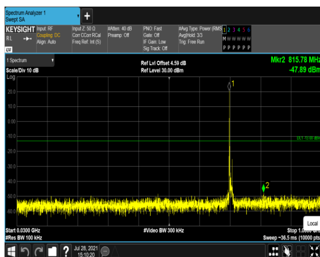
Band12-10MHz-16QAM-23130:30~1000MHz
