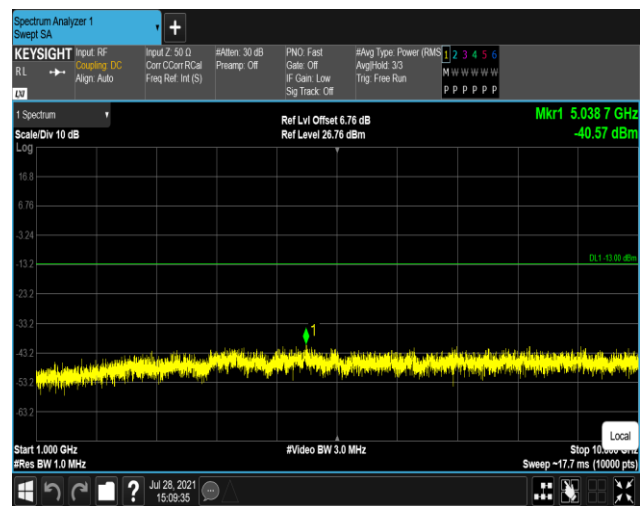
Band12-10MHz-16QAM-23130:1000~10000MHz
