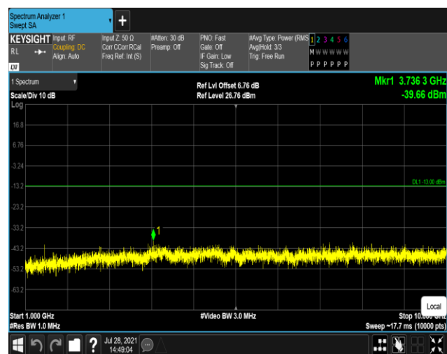
Band12-1.4MHz-QPSK-23173:1000~10000MHz
