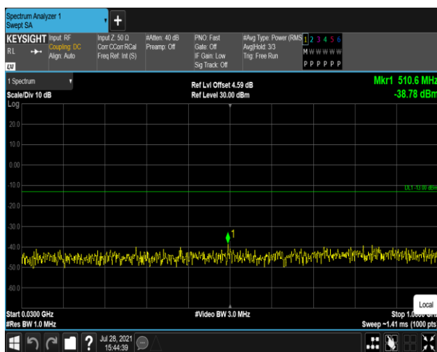
Band25-1.4MHz-QPSK-26683:30~1000MHz
