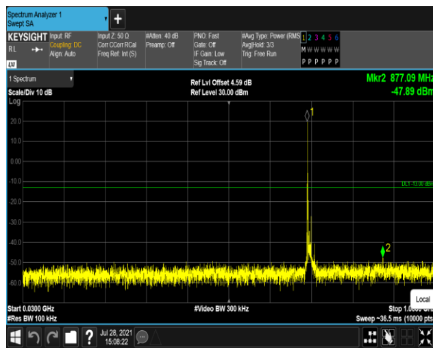
Band12-10MHz-16QAM-23095:30~1000MHz
