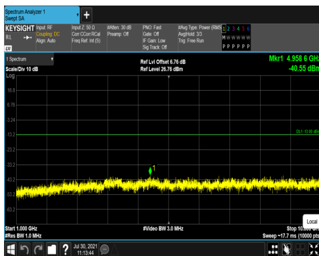
Band13-5MHz-16QAM-23255:1000~10000MHz
