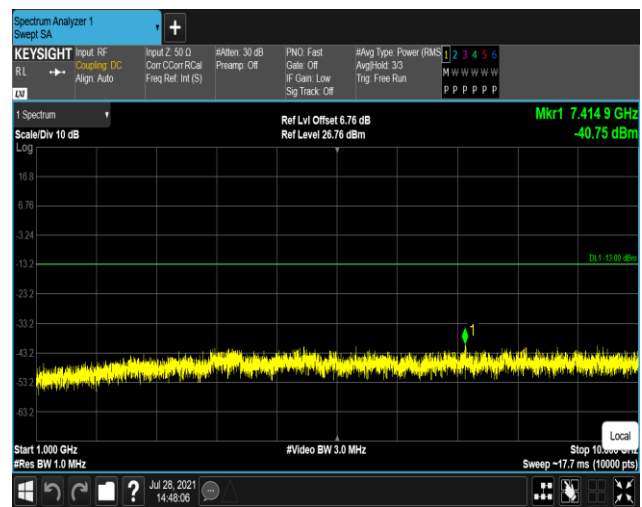
Band12-1.4MHz-16QAM-23095:1000~10000MHz
