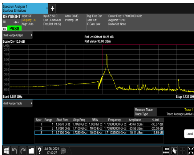
Band66-20MHz-QPSK-132072-100RB#0
