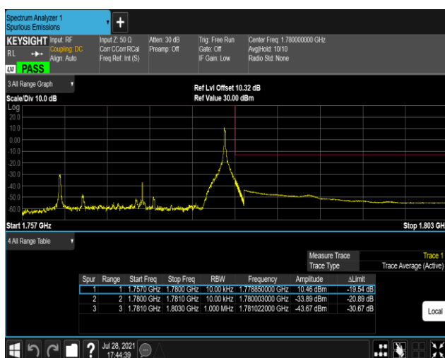
Band66-20MHz-16QAM-132572-1RB#99
