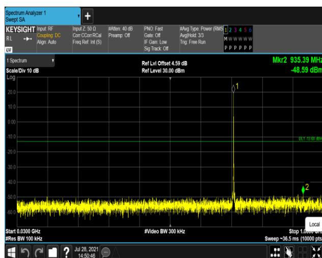
Band12-1.4MHz-16QAM-23173:30~1000MHz
