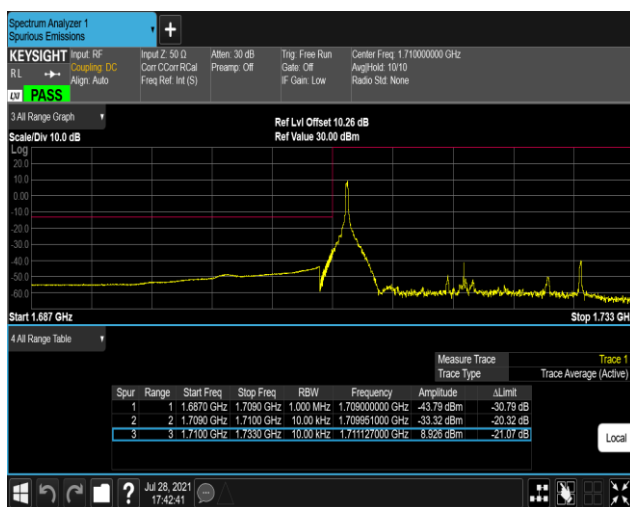
Band66-20MHz-16QAM-132072-100RB#0
