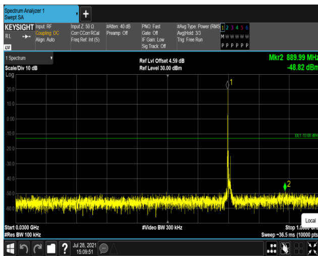
Band12-10MHz-QPSK-23130:30~1000MHz
