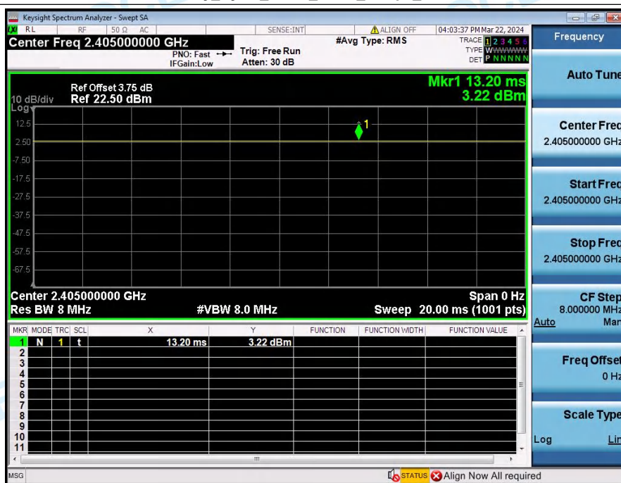
Duty_Cycle_NVNT_ANT1_1Mbps_2405
