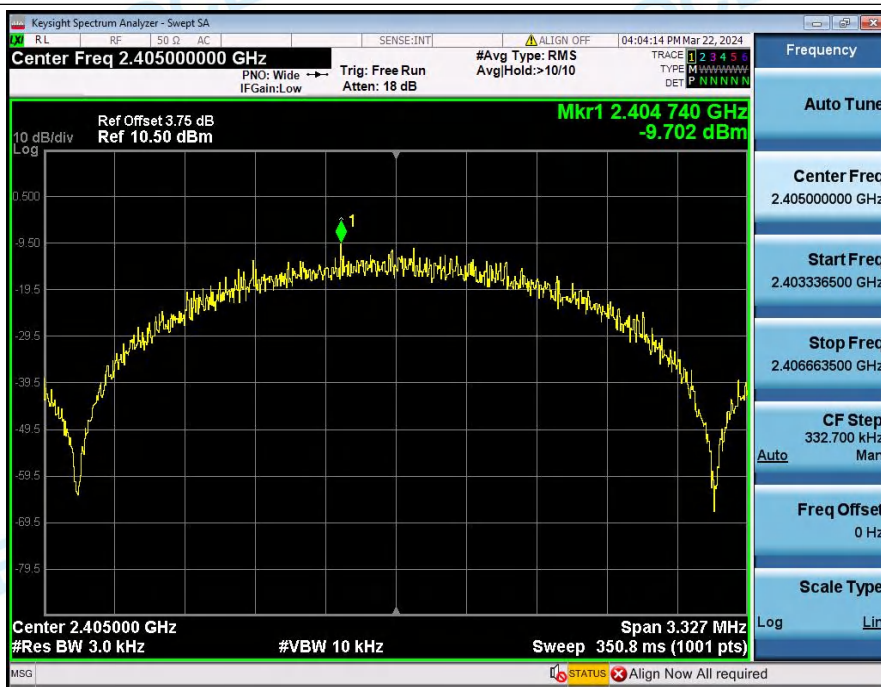
Power_Spectral_Density_NVNT_ANT1_1Mbps_2405
