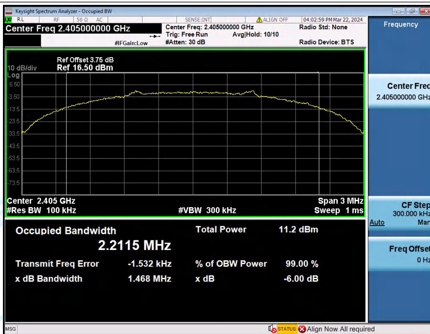
-6dB_Bandwidth_NVNT_ANT1_1Mbps_2405
