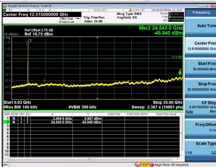
2_Spurious_Emission_NVNT_ANT1_1Mbps_2405
