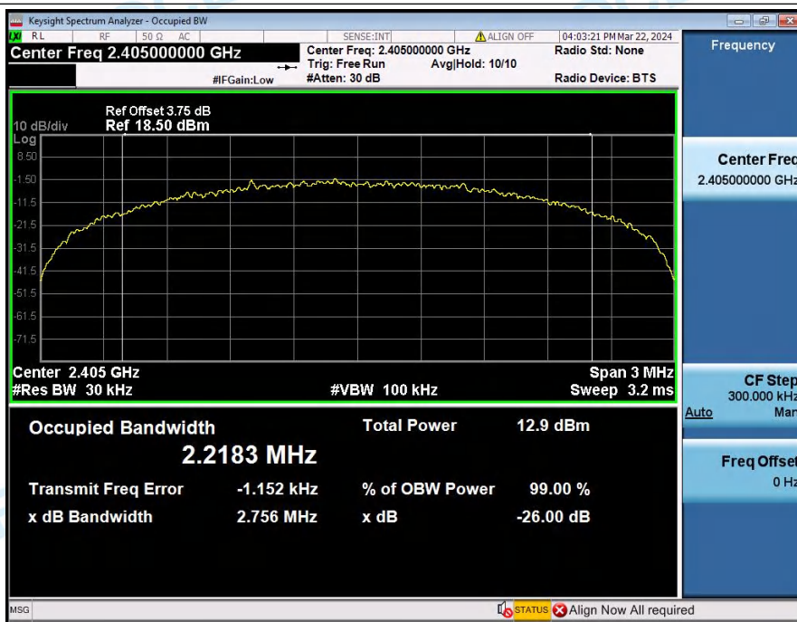
99%_Occupied_Bandwidth_NVNT_ANT1_1Mbps_2405
