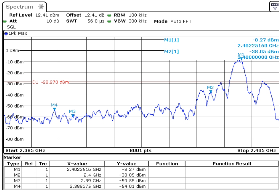
Low Band Edge Plot on Channel 0
