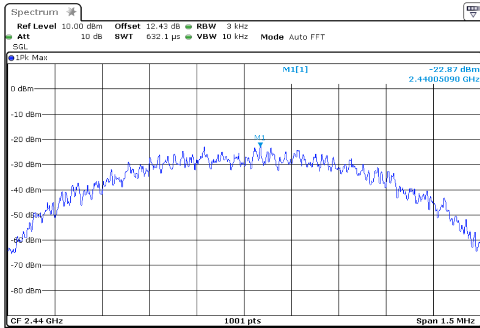
PSD Plot on Channel 19
