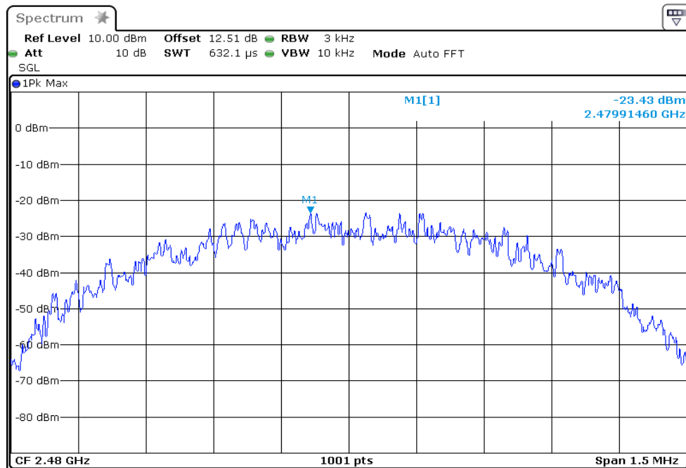
PSD Plot on Channel 39
