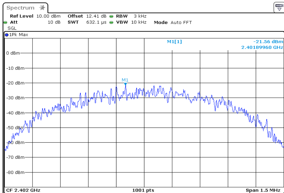
PSD Plot on Channel 0
