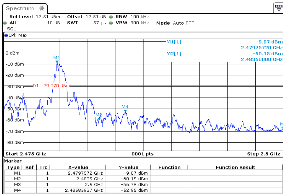
High Band Edge Plot on Channel 39
