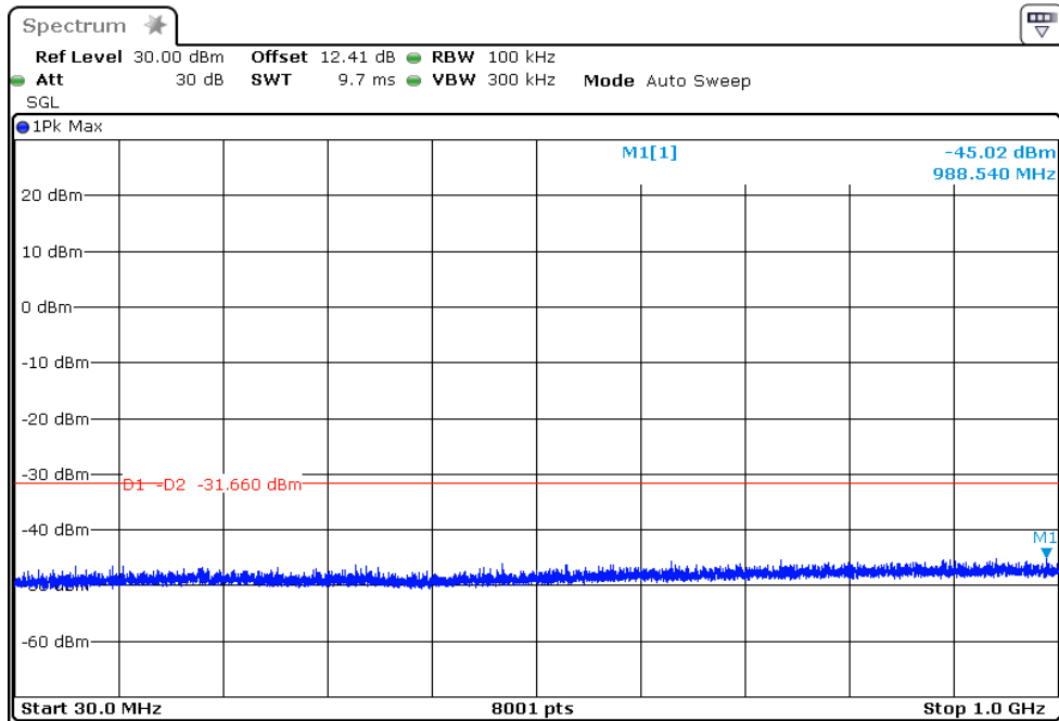
Conducted Spurious Emission Plot on Bluetooth LE 1Mbps
