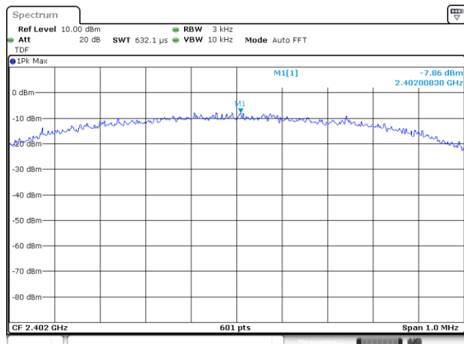
GFSK (BLE) LOW CHANNEL
