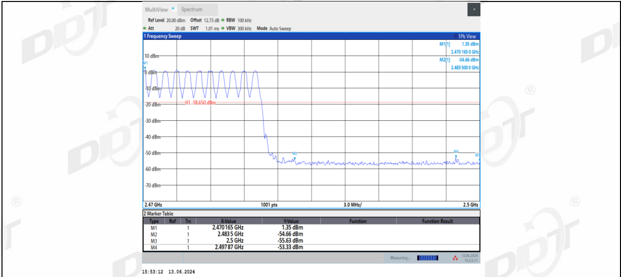
DH5_Right side_High_Hop_2480
