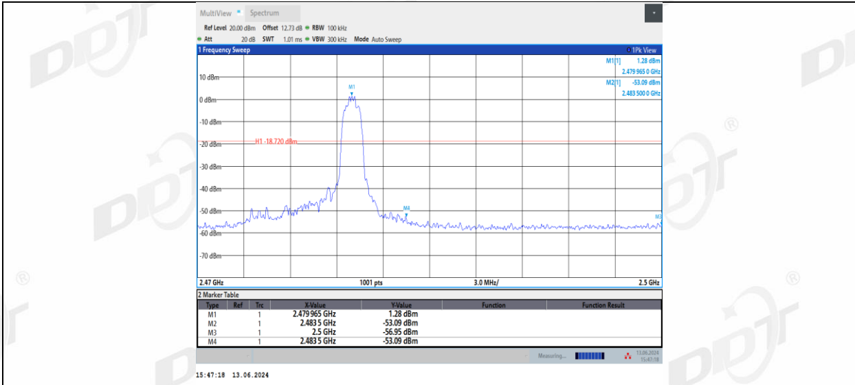
3DH5_Right side_High_2480
