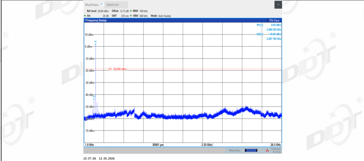
DH5_Right side_2480_0~Reference
