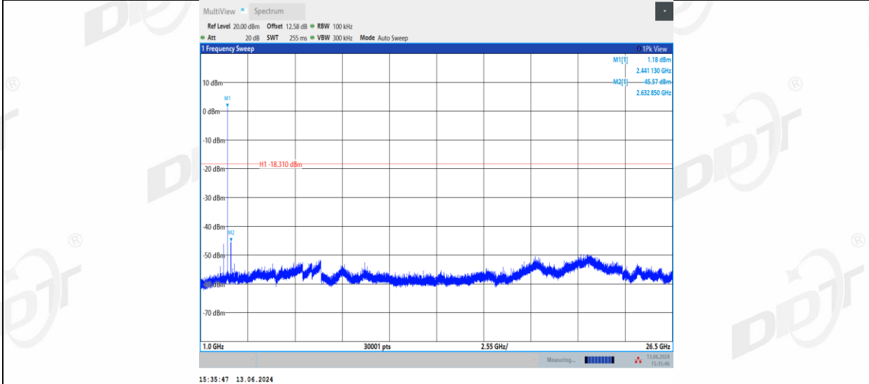
DH5_Right side_2441_0~Reference
