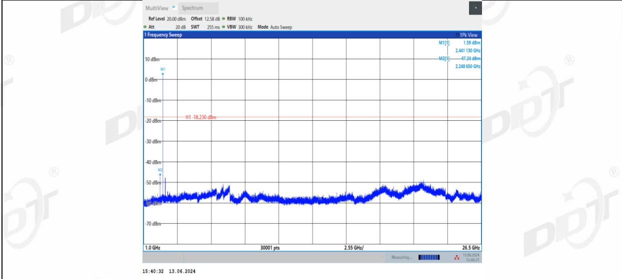
2DH5_Right side_2441_0~Reference
