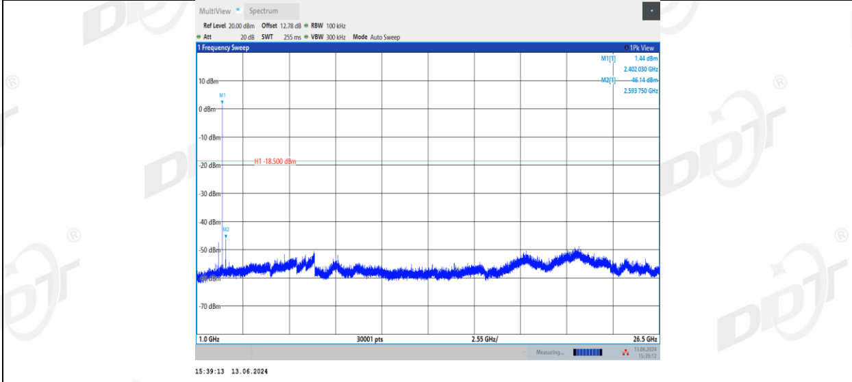
2DH5_Right side_2402_0~Reference
