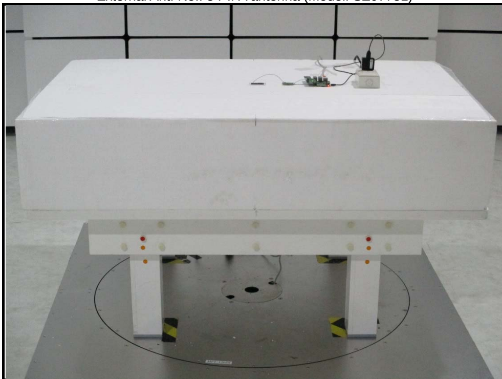
External Ant. No.: 5 PIFA antenna (Model: SZ07751)
