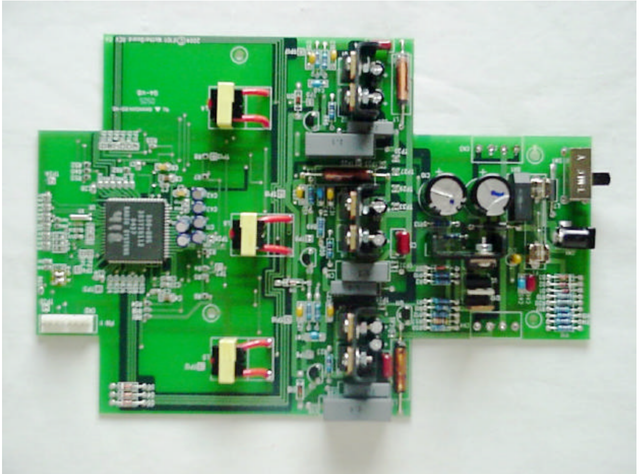
Photo 4. Mother Board, Component Side
