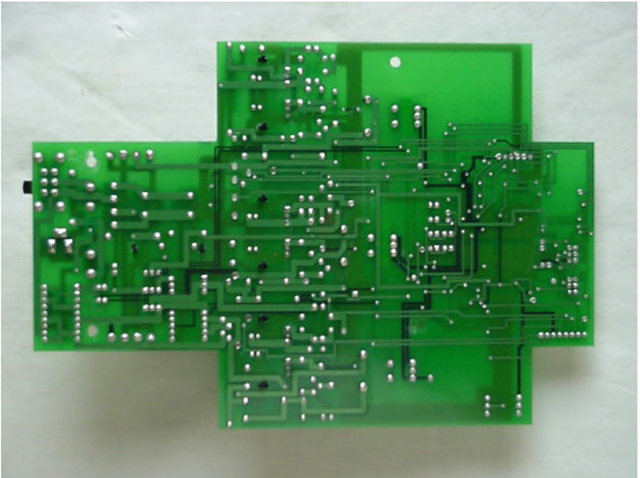
Photo 5. Mother Board, Solder Side
