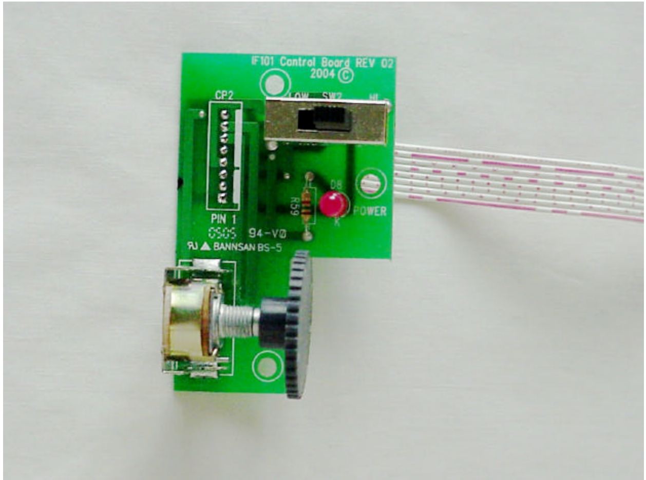
Photo 6. Control Board, Component Side
