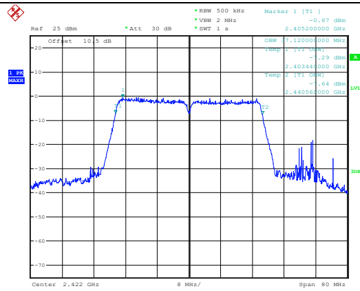
99% Occupied Bandwidth
