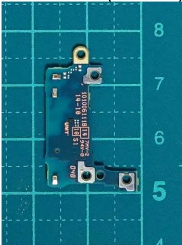
Internal Sub-PWB (Front-side)
