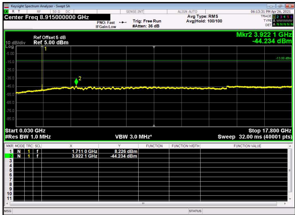
N66(20M)_DFT-s-OFDM_QPSK_Edge_1R B_Left_Low_CH
