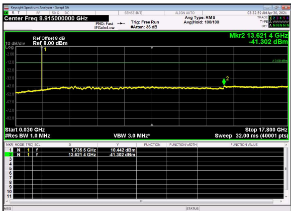
N66(20M)_DFT-s-OFDM_QPSK_Edge_1R B_Left_Mid_CH
