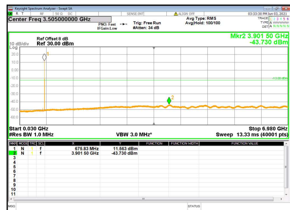
N71(10M)_DFT-s-OFDM_QPSK_Edge_1R B_Left_Mid_CH
