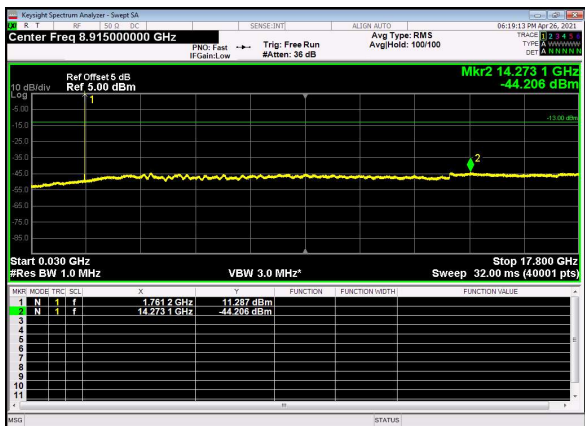
N66(20M)_DFT-s-OFDM_QPSK_Edge_1R B_Left_High_CH
