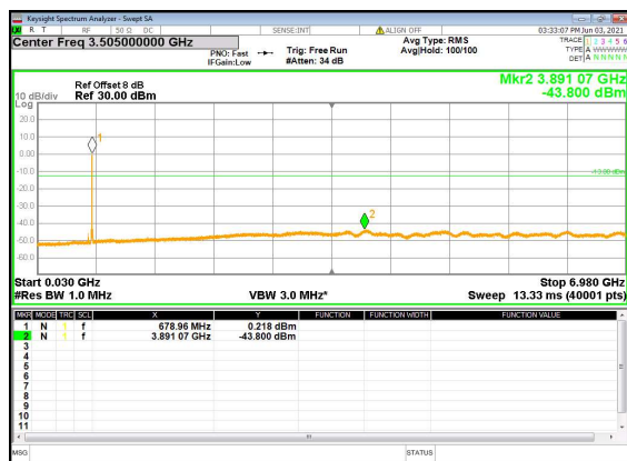
N71(10M)_DFT-s-OFDM_BPSK_Edge_1R B_Left_Mid_CH
