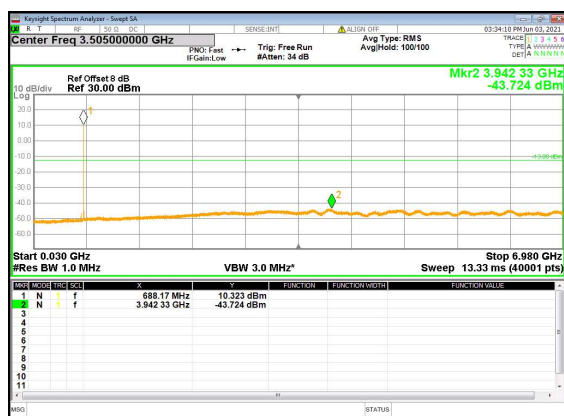
N71(10M)_DFT-s-OFDM_BPSK_Edge_1R B_Left_High_CH
