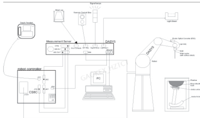
● A standard high precision 6-axis robot (StäubliTX=RX family) with controller, teach pendant and software. An arm extension for accommodating the data acquisition electronics (DAE). ● An isotropic field probe optimized and calibrated for the targeted measurement. ● A data acquisition electronics (DAE) which performs the signal amplification, signal multiplexing, AD-conversion, offset measurements, mechanical surface detection, collision detection, etc. The unit is battery powered with standard or rechargeable batteries. The signal is optically transmitted to the EOC. ● The Electro-optical converter (EOC) performs the conversion from optical to electrical signals for the digital communication to the DAE. To use optical surface detection, a special version of the EOC is required. The EOC signal is transmitted to the measurement server. ● The function of the measurement server is to perform the time critical tasks such as signal filtering, control of the robot operation and fast movement interrupts. ● The Light Beam used is for probe alignment. This improves the (absolute) accuracy of the probe positioning. ● A computer running WinXP and the DASY4 or DASY5 software. ● Remote control and teach pendant as well as additional circuitry for robot safety such as warning lamps, etc. ● The phantom, the device holder and other accessories according to the targeted measurement.
