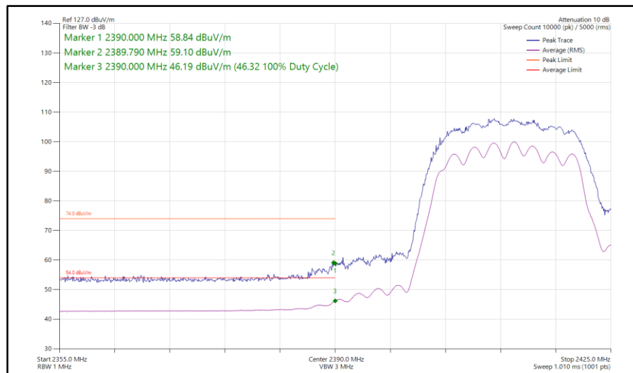
Figure 61 - 802.11n HT20, CDD, Core 0-1 - 2412 MHz Band Edge Frequency 2390 MHz
