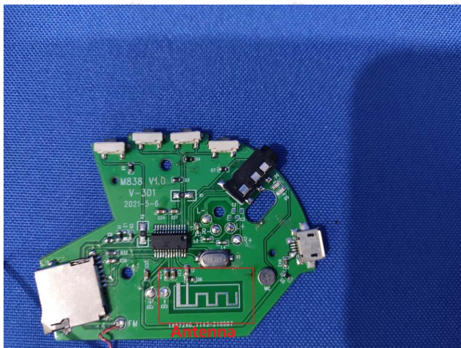
View of Product-16 (Antenna)
