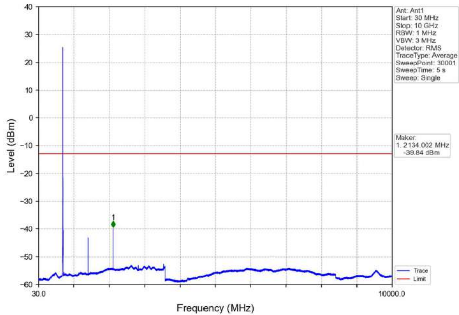
Band17_5MHz_QPSK_HCH_713.5MHz_RB_1_0_NTNV
