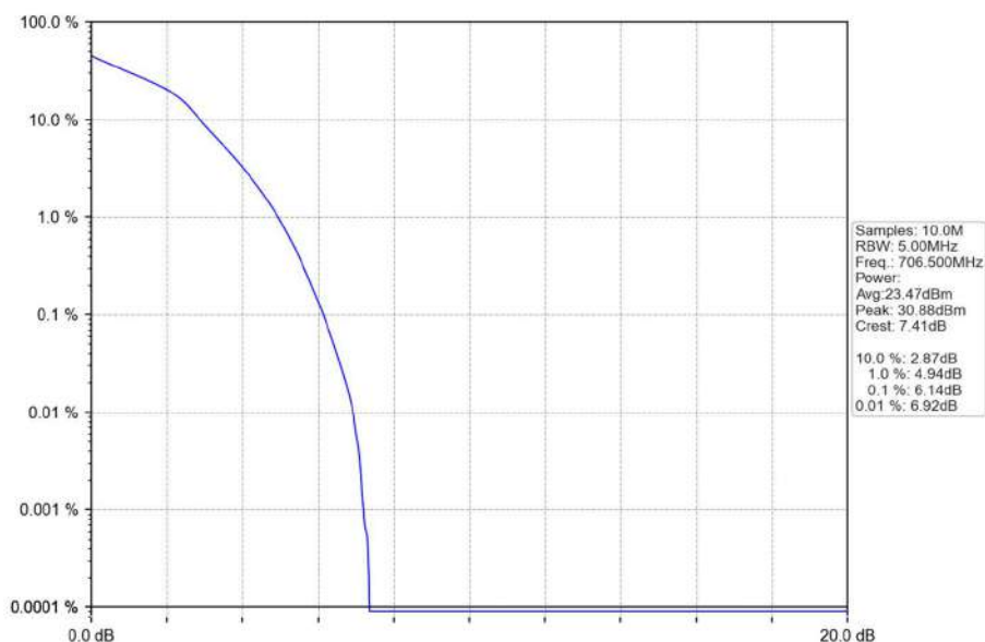
Band17_5MHz_16QAM_LCH_706.5MHz_RB_25_0_NTNV
