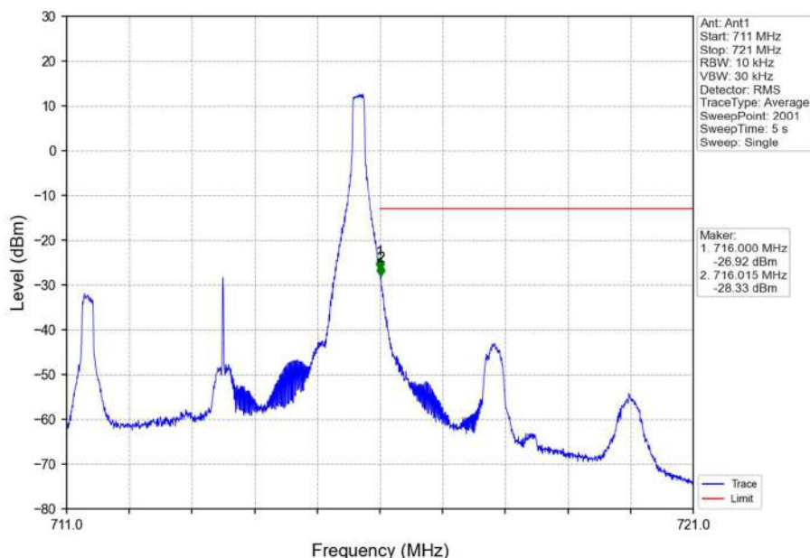
Band17_5MHz_16QAM_HCH_713.5MHz_RB_1_24_NTNV
