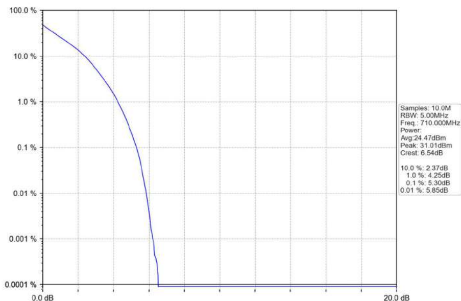
Band17_5MHz_QPSK_MCH_710MHz_RB_25_0_NTNV
