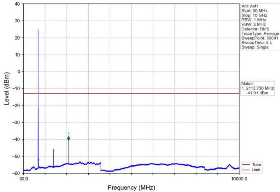
Band17 10MHz 16QAM LCH 709MHz RB 1 0 NTV
