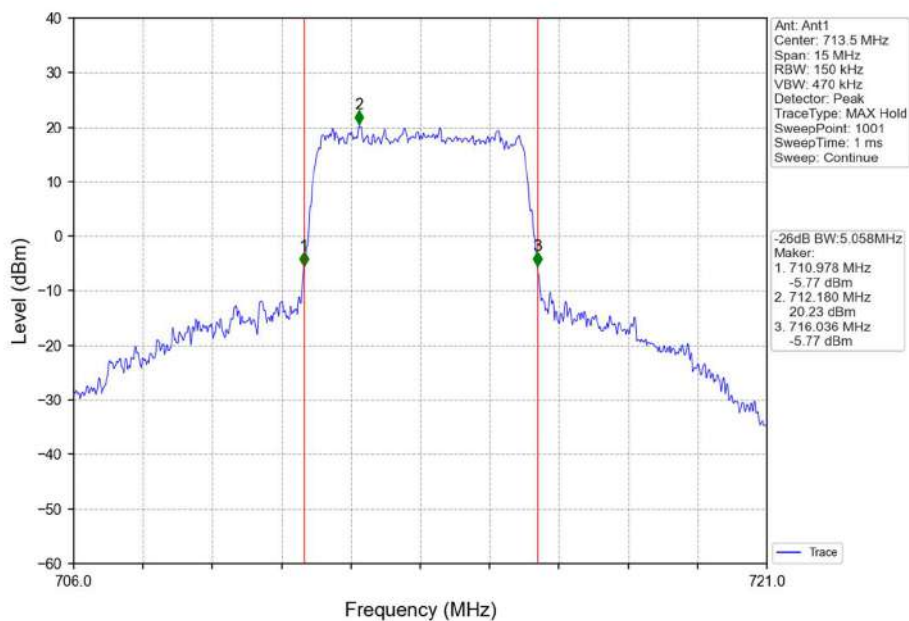
Band17_5MHz_16QAM_HCH_713.5MHz_RB_25_0_NTNV
