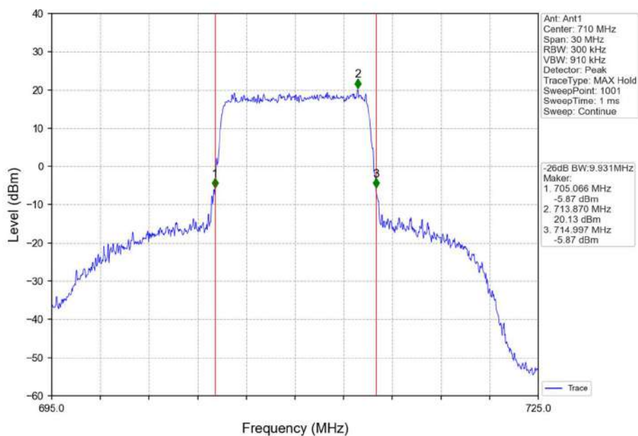
Band17 10MHz 16QAM MCH 710MHz RB 50 0 NTNV
