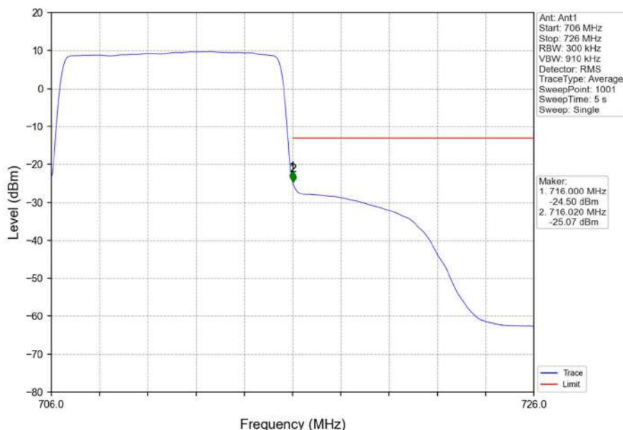
Band17_10MHz_16QAM_HCH_711MHz_RB_50_0_NTNV
