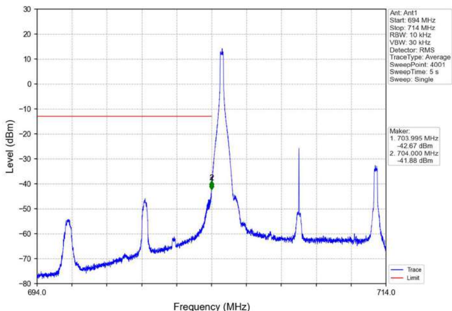
Band17_10MHz_16QAM_LCH_709MHz_RB_1_0_NTNV
