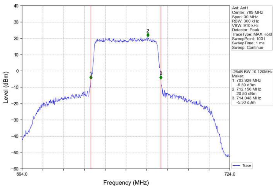
Band17 10MHz QPSK LCH 709MHz RB 50 0 NTNV
