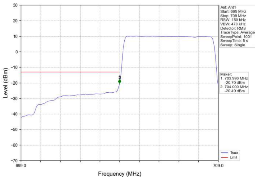
Band17_5MHz_QPSK_LCH_706.5MHz_RB_25_0_NTNV
