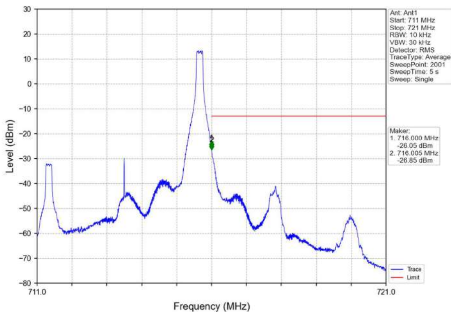
Band17_5MHz_QPSK_HCH_713.5MHz_RB_1_24_NTNV
