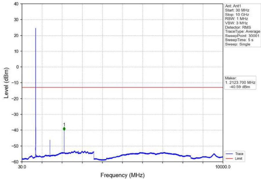
Band17_5MHz_16QAM_MCH_710MHz_RB_1_0_NTNV
