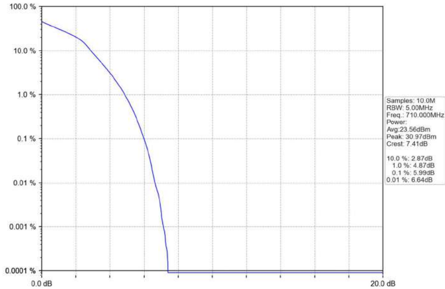
Band17_5MHz_16QAM_MCH_710MHz_RB_25_0_NTNV
