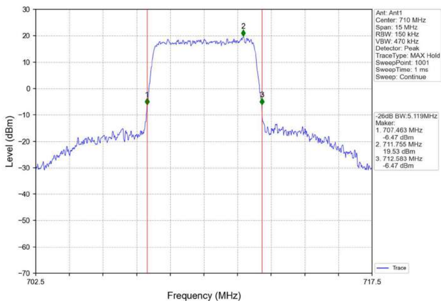
Band17 5MHz 16QAM MCH 710MHz RB 25 0 NTNV
