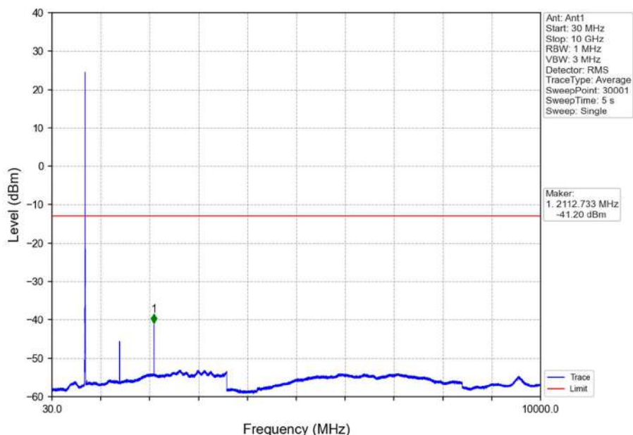
Band17_5MHz_16QAM_LCH_706.5MHz_RB_1_0_NTNV
