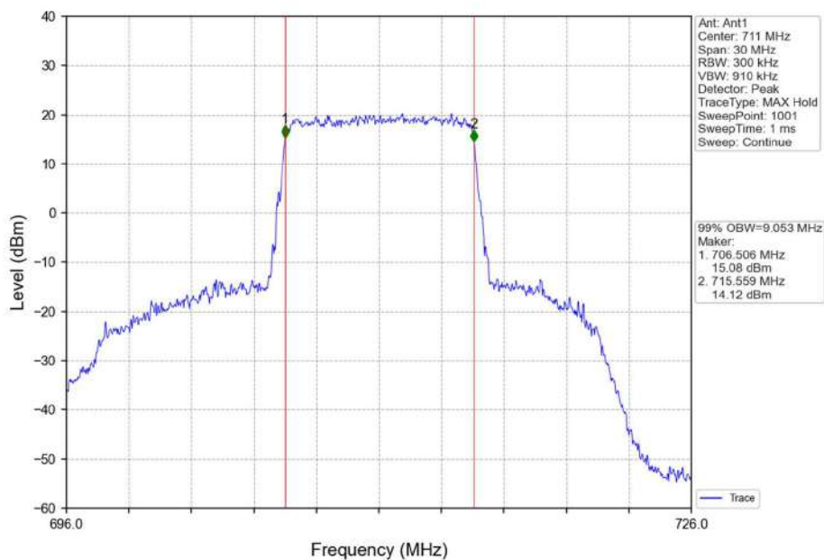
Band17_10MHz_QPSK_HCH_711MHz_RB_50_0_NTNV
