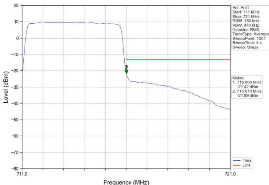
Band17_5MHz_16QAM_HCH_713.5MHz_RB_25_0_NTNV
