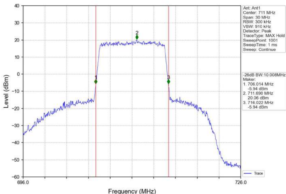
Band17_10MHz_16QAM_HCH_711MHz_RB_50_0_NTNV
