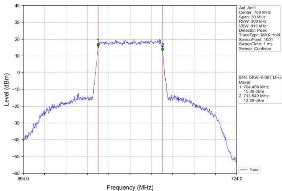
Band17_10MHz_16QAM_LCH_709MHz_RB_50_0_NTNV
