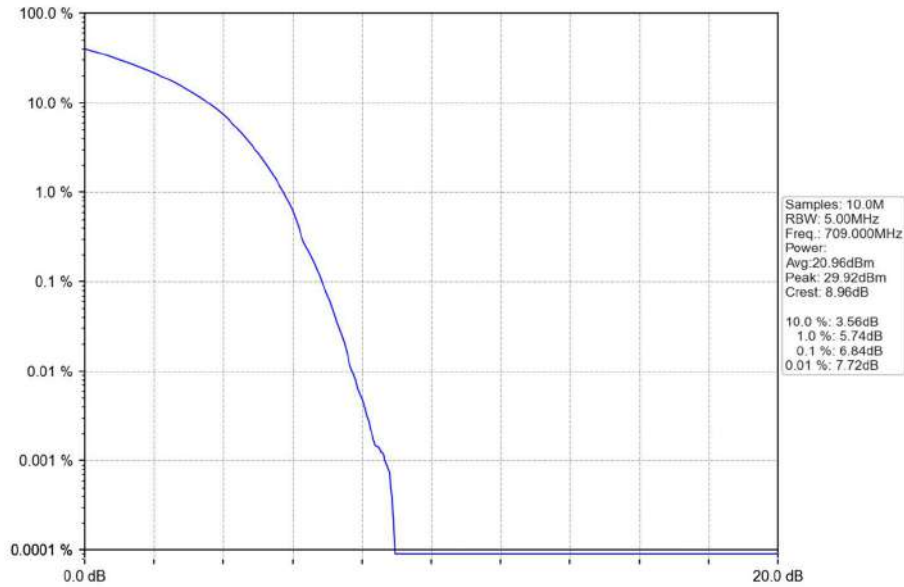
Band17_10MHz_16QAM_LCH_709MHz_RB_50_0_NTNV
