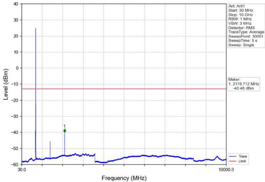
Band17_10MHz_16QAM_HCH_711MHz_RB_1_0_NTNV
