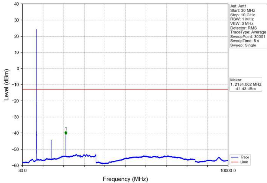
Band17_5MHz_16QAM_HCH_713.5MHz_RB_1_0_NTNV
