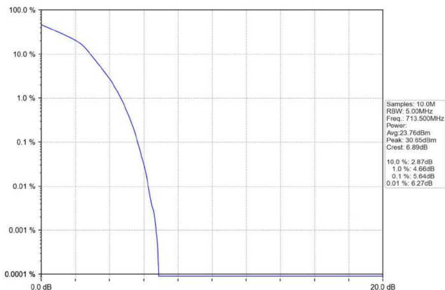
Band17_5MHz_16QAM_HCH_713.5MHz_RB_25_0_NTNV
