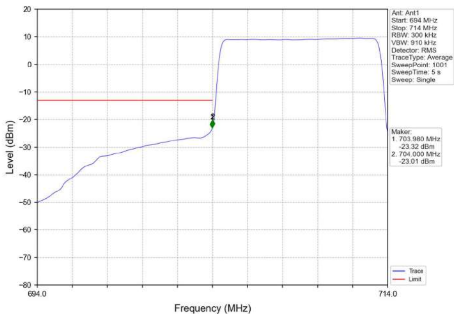
Band17_10MHz_16QAM_LCH_709MHz_RB_50_0_NTNV
