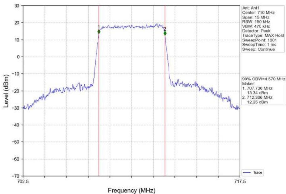
Band17_5MHz_16QAM_MCH_710MHz_RB_25_0_NTNV
