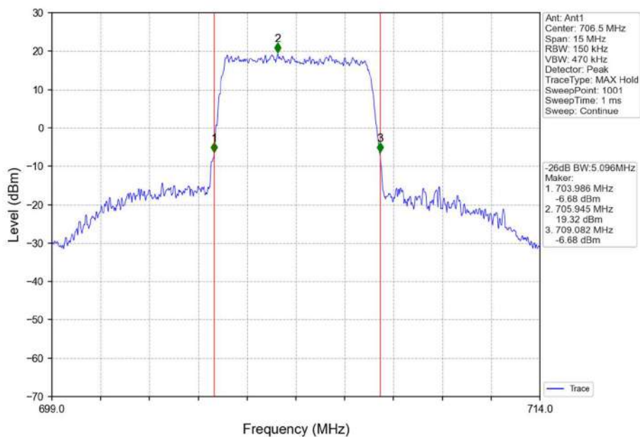
Band17_5MHz_16QAM_LCH_706.5MHz_RB_25_0_NTNV
