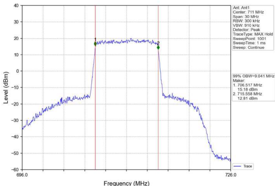
Band17_10MHz_16QAM_HCH_711MHz_RB_50_0_NTNV
