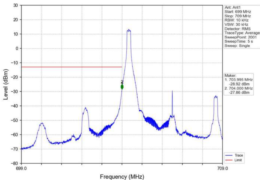
Band17_5MHz_16QAM_LCH_706.5MHz_RB_1_0_NTNV
