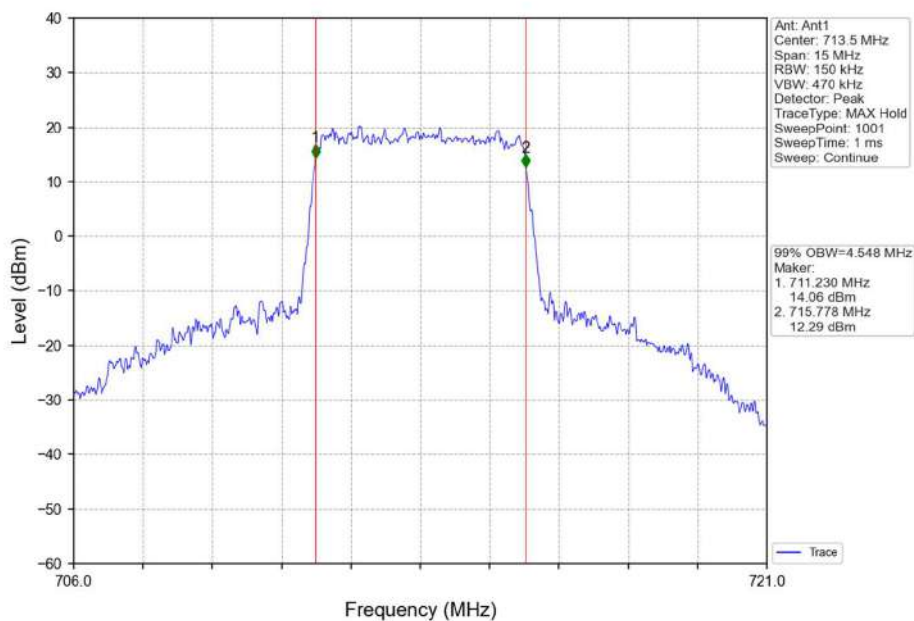
Band17_5MHz_16QAM_HCH_713.5MHz_RB_25_0_NTNV
