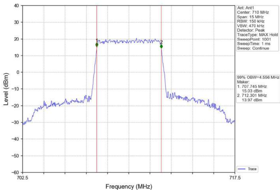
Band17_5MHz_QPSK_MCH_710MHz_RB_25_0_NTNV
