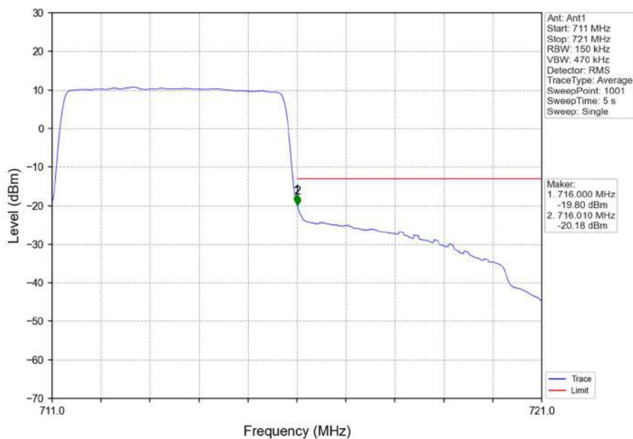
Band17_5MHz_QPSK_HCH_713.5MHz_RB_25_0_NTNV
