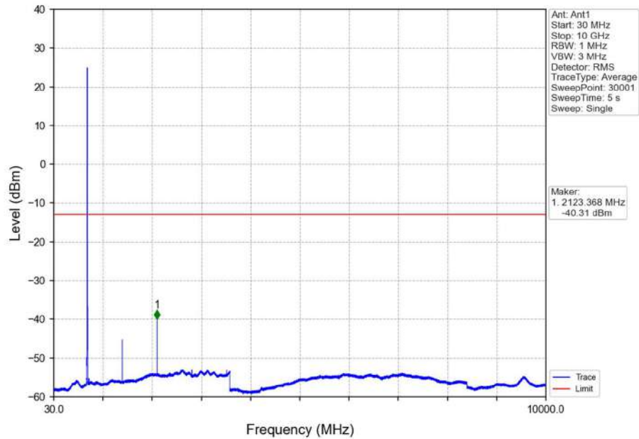
Band17_5MHz_QPSK_MCH_710MHz_RB_1_0_NTNV
