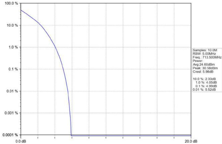
Band17_5MHz_QPSK_HCH_713.5MHz_RB_25_0_NTNV
