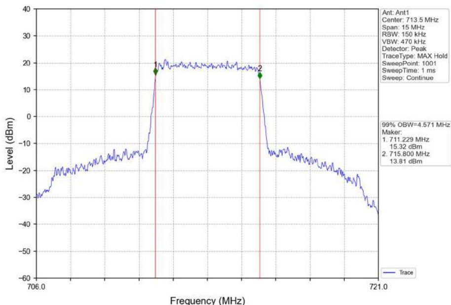
Band17_5MHz_QPSK_HCH_713.5MHz_RB_25_0_NTNV
