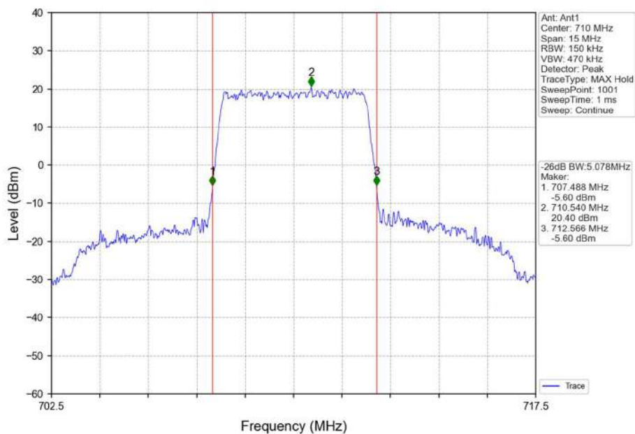
Band17_5MHz_QPSK_MCH_710MHz_RB_25_0_NTNV
