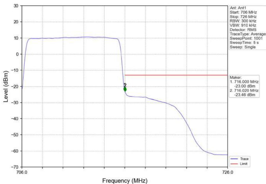
Band17 10MHz QPSK HCH 711MHz RB 50 0 NTNV
