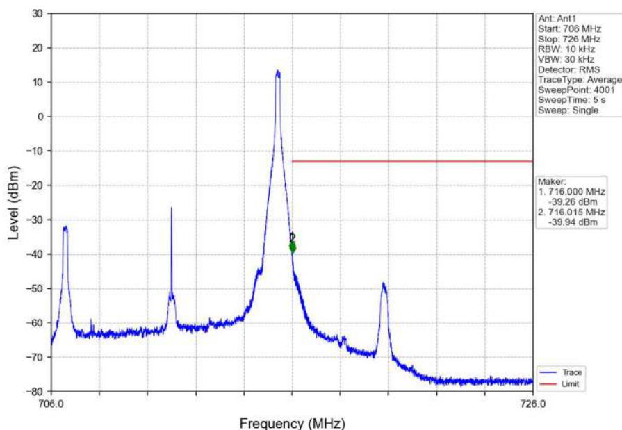
Band17 10MHz 16QAM HCH 711MHz RB 1 49 NTN
