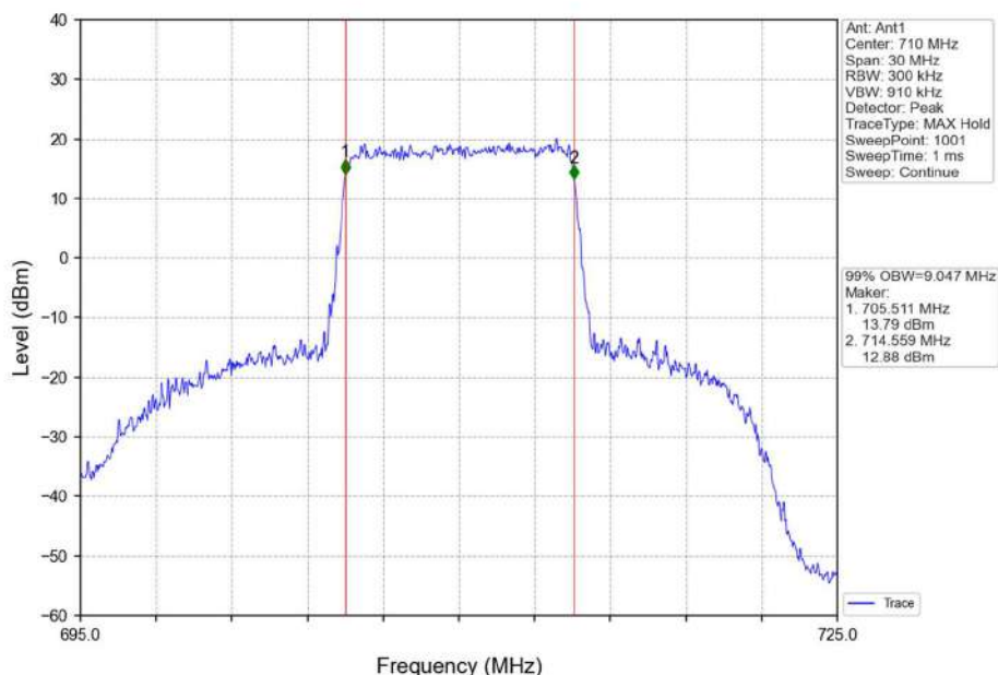
Band17_10MHz_16QAM_MCH_710MHz_RB_50_0_NTNV
