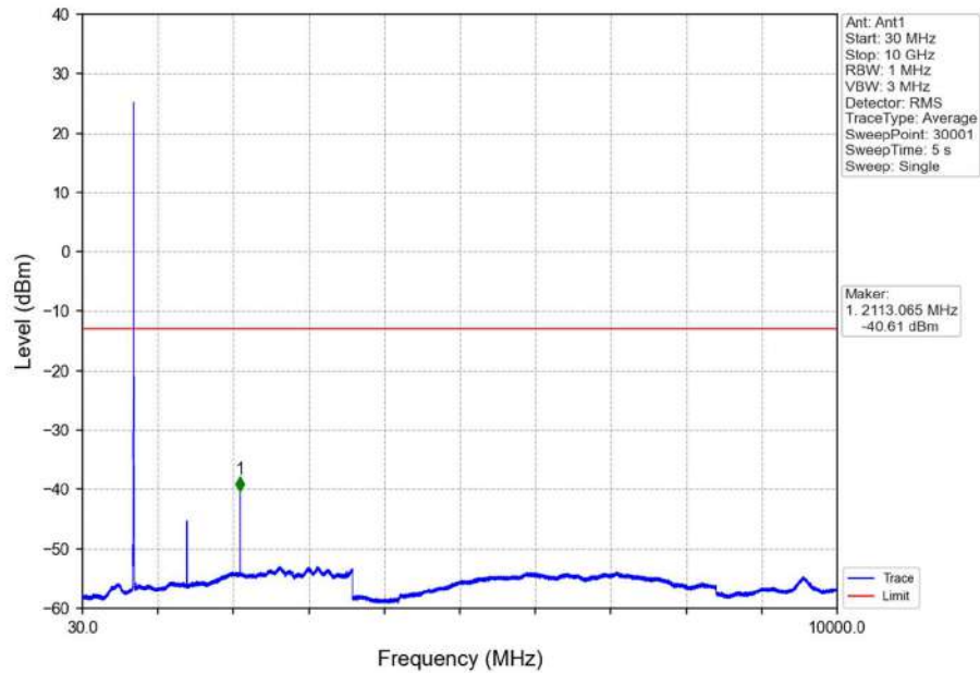
Band17_5MHz_QPSK_LCH_706.5MHz_RB_1_0_NTNV
