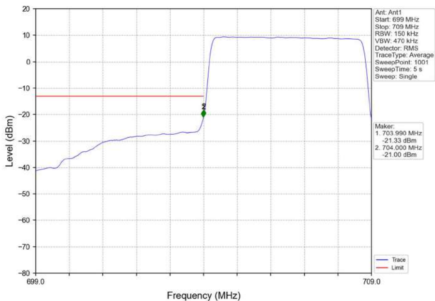
Band17_5MHz_16QAM_LCH_706.5MHz_RB_25_0_NTNV
