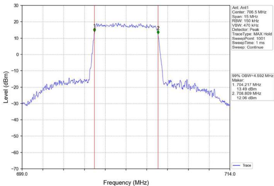
Band17_5MHz_16QAM_LCH_706.5MHz_RB_25_0_NTNV
