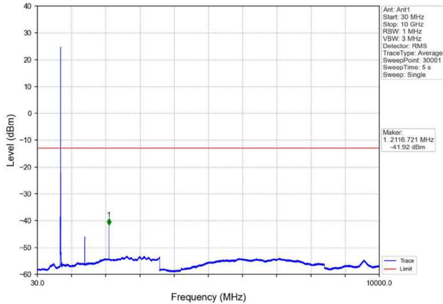
Band17 10MHz 16QAM MCH 710MHz RB 1 0 NTNV
