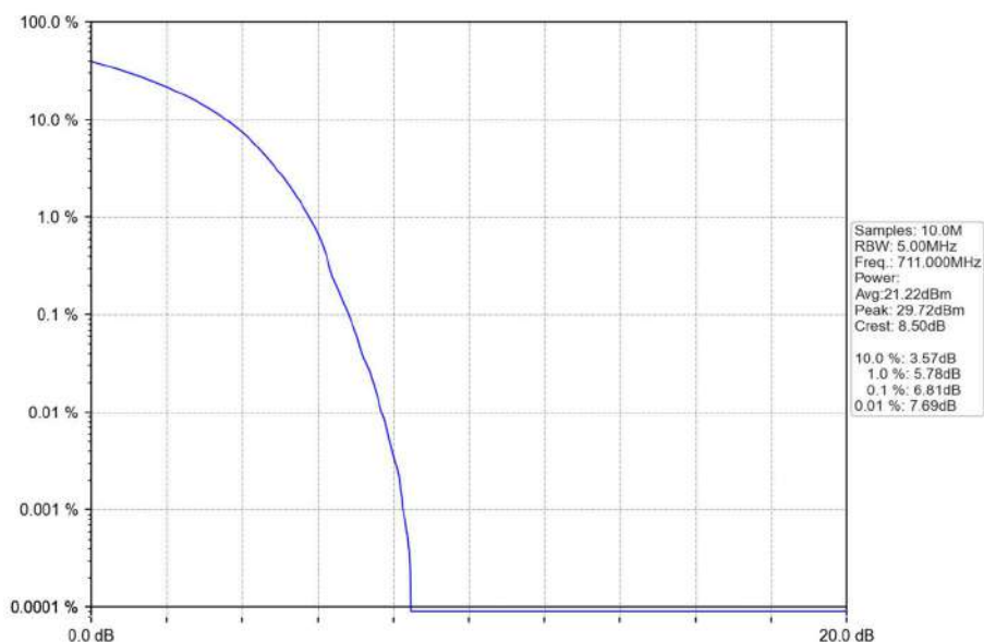
Band17_10MHz_16QAM_HCH_711MHz_RB_50_0_NTNV
