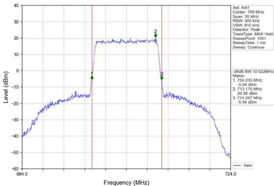
Band17_10MHz_16QAM_LCH_709MHz_RB_50_0_NTNV
