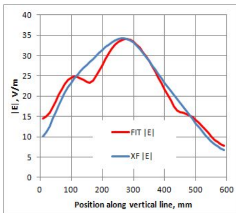
Electric field magnitude (870MHz)
