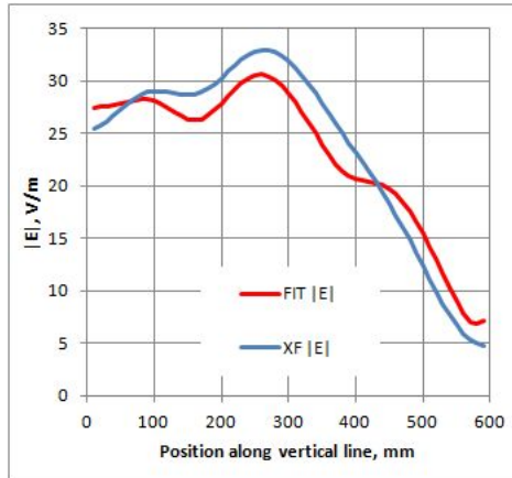
Electric field magnitude (764 MHz)
