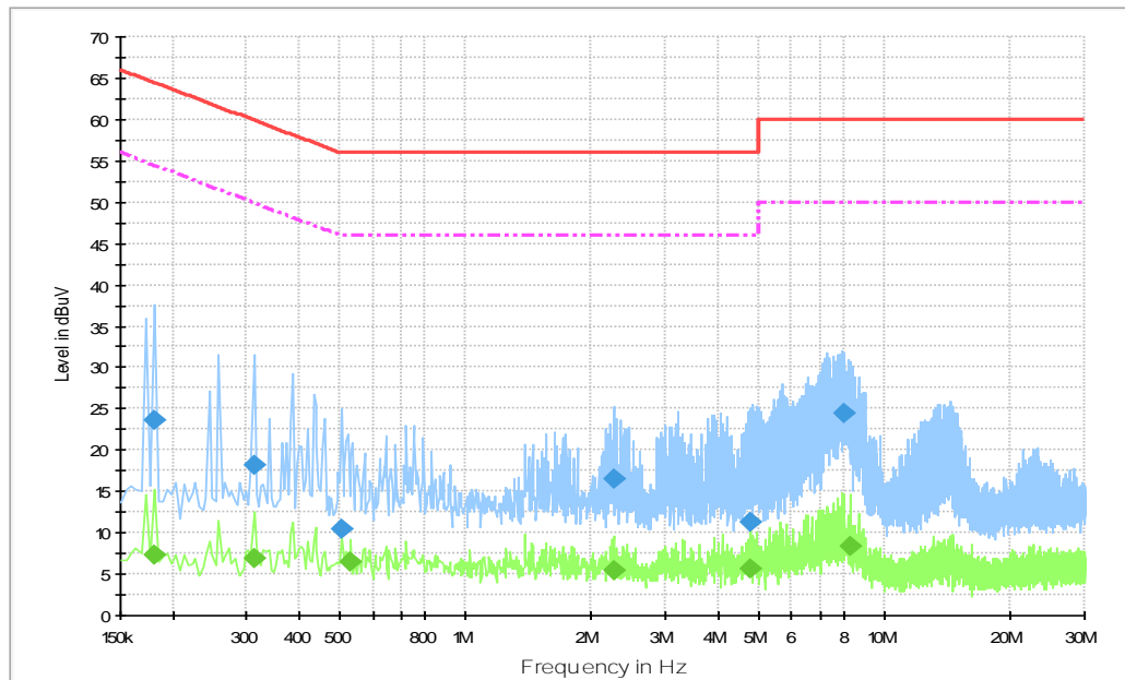
Fig.B.8.2 AC Powerline Conducted Emission-Iidle
