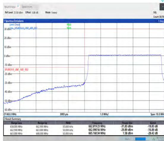
1-N71-PC3-15-5-L-6-CP-QPSK-Outer_Full-25@0 Ant1-1--PASS-see graph
