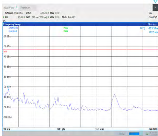
1-N71-PC3-15-20-M-1-DFT-QPSK-Inner_1RB_Left-1 @1-0.009-0.15-Ant1-0.01--73.37--33-PASS
