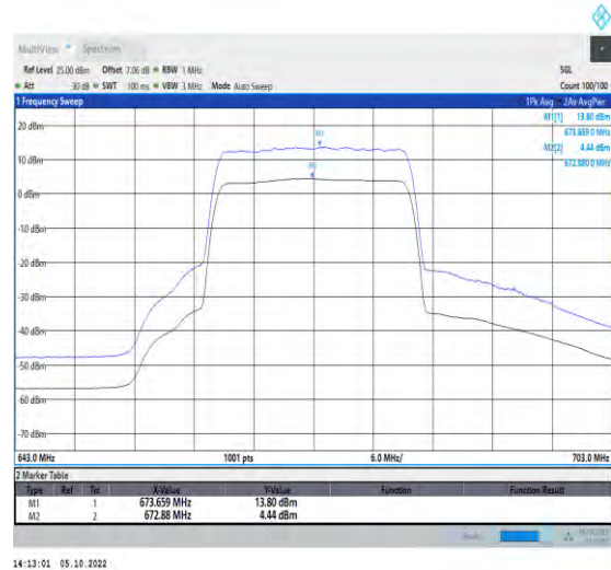
1-N71-PC3-15-20-L-2-CP-256QAM-Outer_Full-106 @0-Ant1-9.36-100%-0.00-9.36-PASS-≤13
