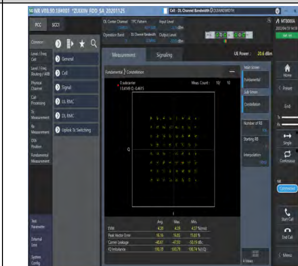
1-N71--15-20-M-8-CP-64QAM-Outer_Full-106@0-Ant1-see graph-PASS
