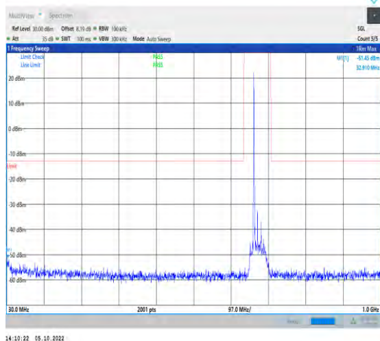
1-N71-PC3-15-20-L-1-DFT-QPSK-Inner_1RB_Left-1 @1-30-1000-Ant1-34.85--51.52--13-PASS
