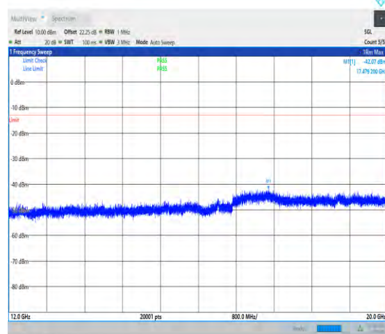
1-N71-PC3-15-20-L-1-DFT-QPSK-Inner_1RB_Left-1 @1-12000-20000-Ant1-17479.20--42.07--13-PASS
