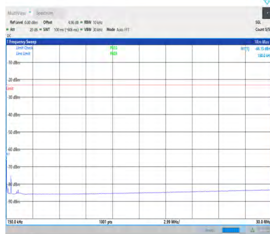
1-N71-PC3-15-20-M-1-DFT-QPSK-Inner_1RB_Left-1 @1-0.15-30-Ant1-0.15--66.15--23-PASS
