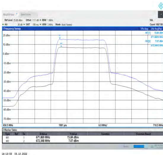
1-N71-PC3-15-20-M-1-DFT-256QAM-Outer_Full-100 @0-Ant1-8.77-100%-0.00-8.77-PASS-≤13
