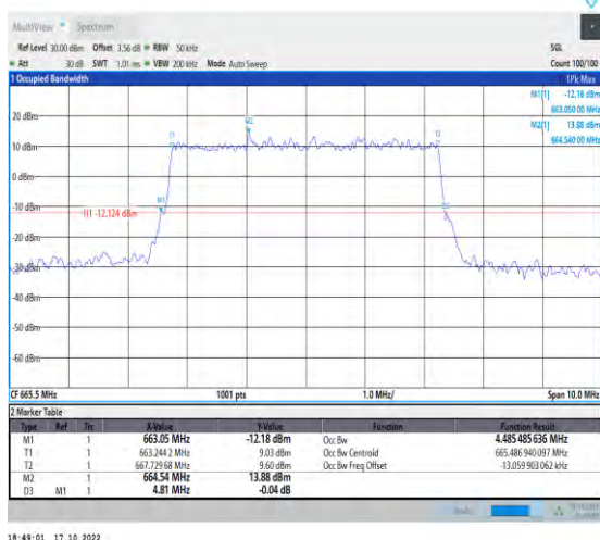
1-N71-PC3-15-5-L-1-DFT-QPSK-Outer_Full-25@0- Ant1-4.485-4.810-≤5-PASS
