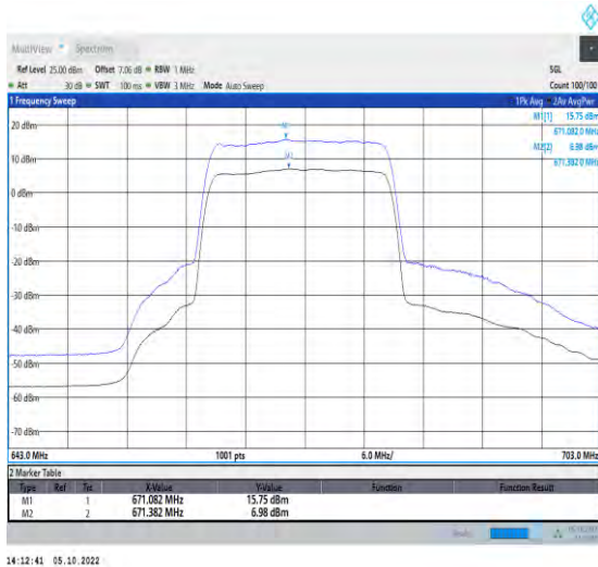
1-N71-PC3-15-20-L-1-DFT-256QAM-Outer_Full-100 @0-Ant1-8.77-100%-0.00-8.77-PASS-≤13
