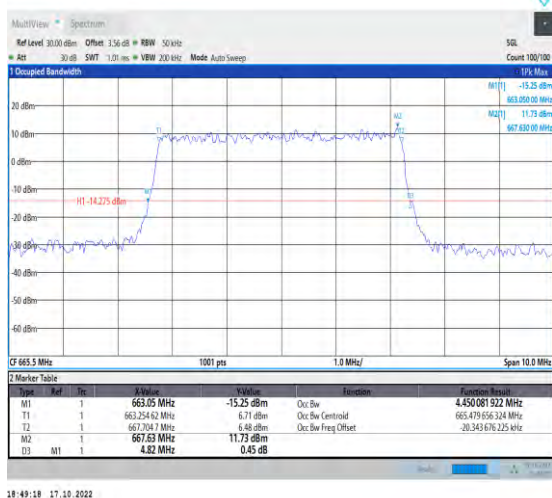
1-N71-PC3-15-5-L-4-DFT-64QAM-Outer_Full-25@0- -Ant1-4.45-4.820-≤5-PASS
