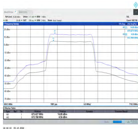
1-N71-PC3-15-20-M-2-CP-256QAM-Outer_Full-106 @0-Ant1-9.44-100%-0.00-9.44-PASS-≤13
