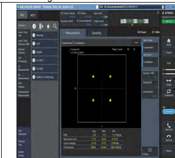
1-N71--15-20-M-6-CP-QPSK-Outer_Full-106@0-Ant1-see graph-PASS
