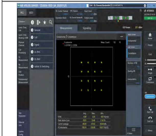
1-N71--15-20-M-7-CP-16QAM-Outer_Full-106@0-Ant1-see graph-PASS
