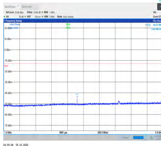
1-N71-PC3-15-20-L-1-DFT-QPSK-Inner_1RB_Left-1 @1-1000-3000-Ant1-1922.00--44.27--13-PASS
