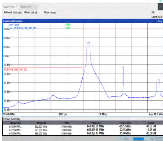
1-N71-PC3-15-5-L-4-CP-QPSK-Edge_1RB_Left-1@0 Ant1-1--PASS-see graph
