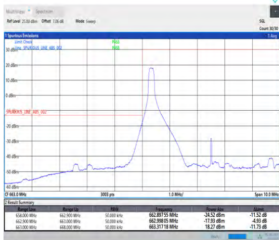
1-N71-PC3-15-5-L-1-DFT-QPSK-Edge_1RB_Left-1@0 -Ant1-1--PASS-see graph
