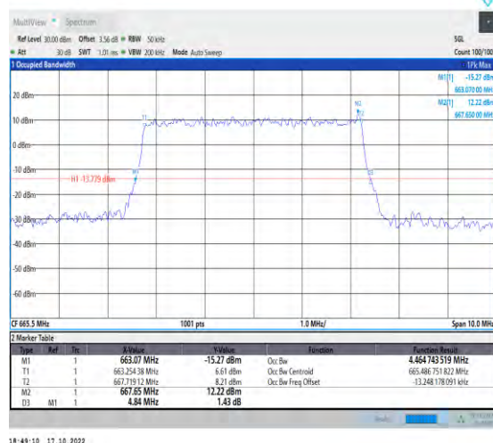
1-N71-PC3-15-5-L-3-DFT-16QAM-Outer_Full-25@0- Ant1-4.465-4.840-≤5-PASS
