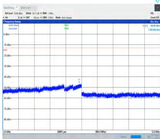
1-N71-PC3-15-20-L-1-DFT-QPSK-Inner_1RB_Left-1 @1-3000-12000-Ant1-7360.50--45.85--13-PASS
