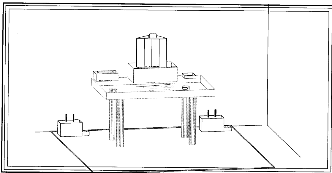
Fig. 10. System Setup.
