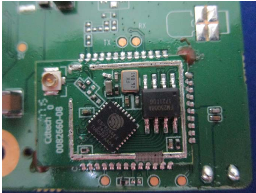
EUT – RF Module Unshielded View
