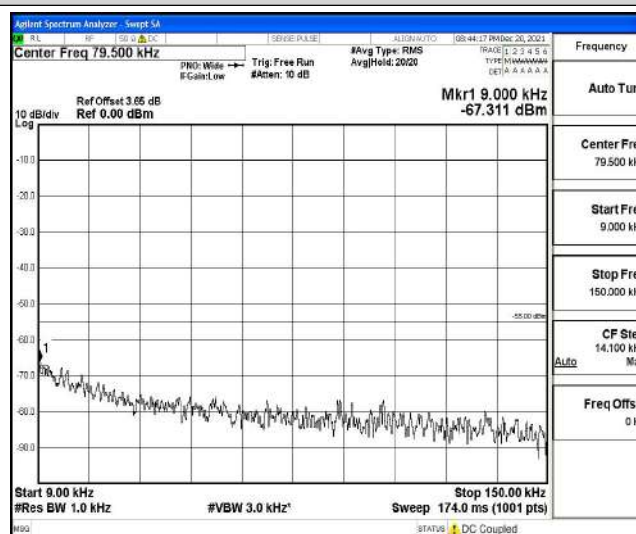
Band38-10MHz-16QAM-38000-1RB#0-Range2:0.15~30MHz
