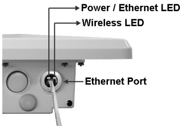
Figure 3-50 View LEDs
