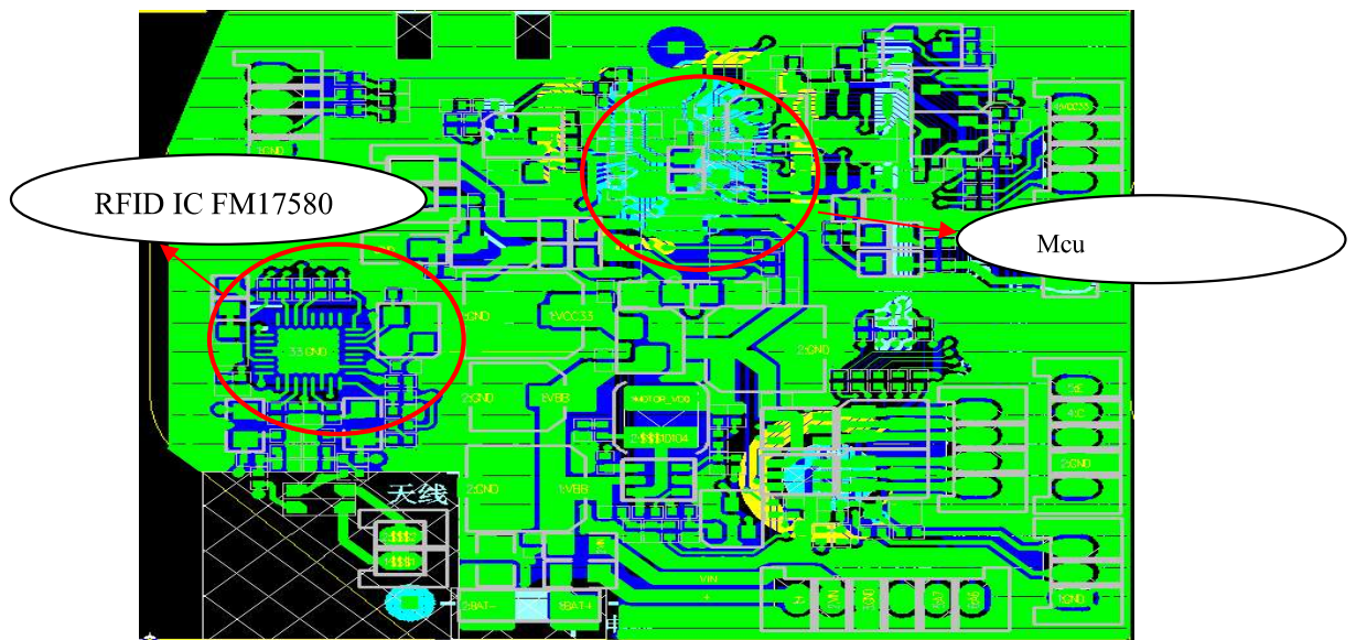
Figure 2.1 RFID module layout for 5601xx main board unit
