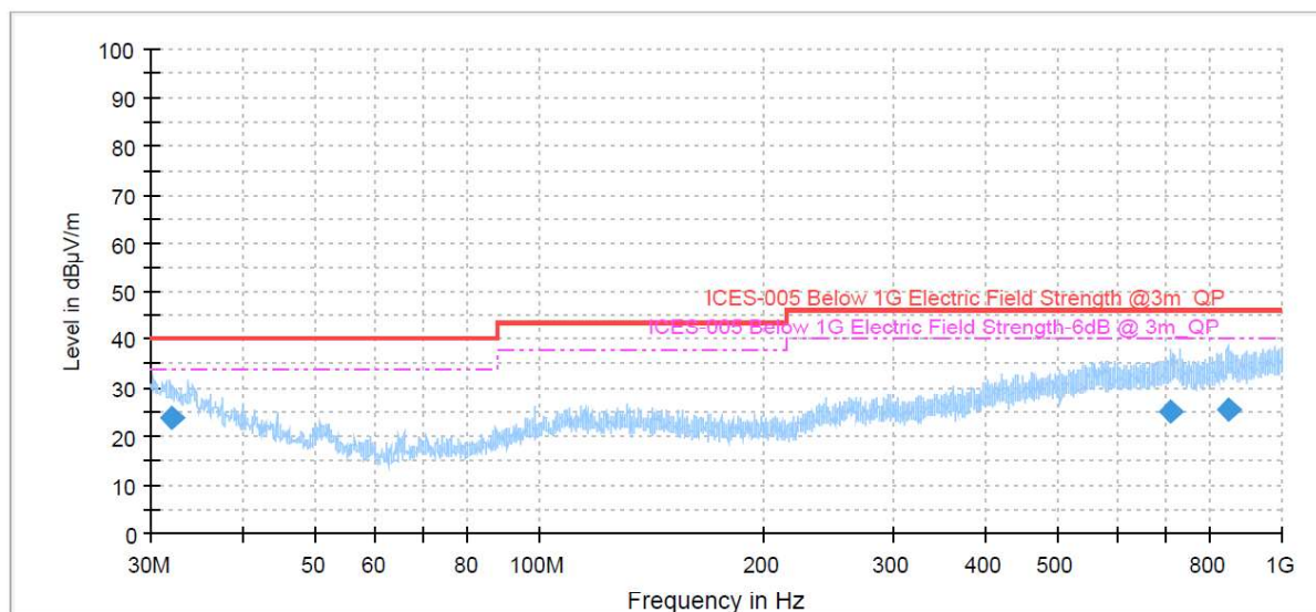
Figure 4: Spectral Diagrams, Radiated Emission, 30MHz-1000MHz, Vertical polarization
