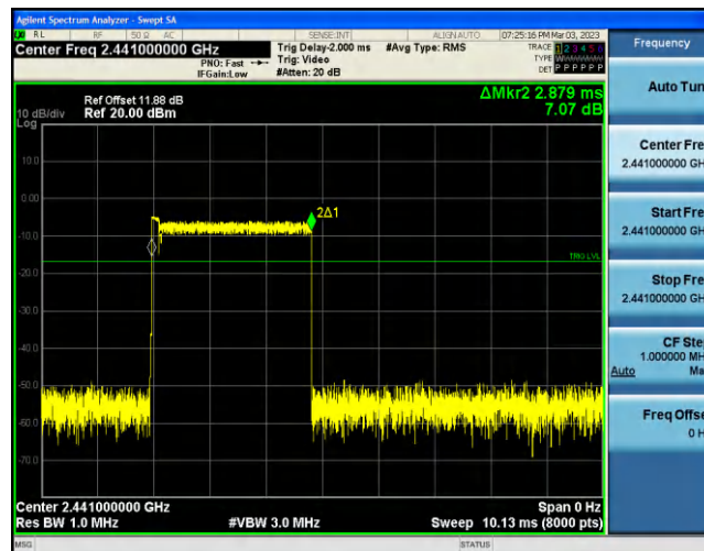
2DH1-Ant1-Hop-0.380-320
