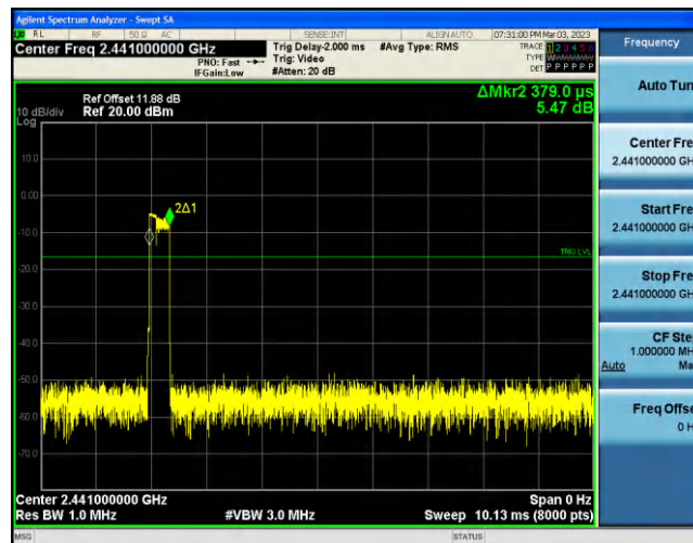
3DH3-Ant1-Hop-1.630-160
