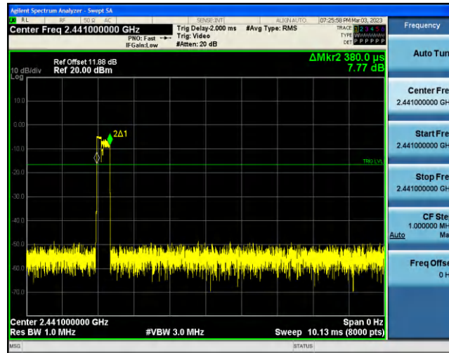
2DH3-Ant1-Hop-1.631-160
