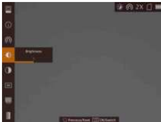
Figure 2-1 Menu Interface
