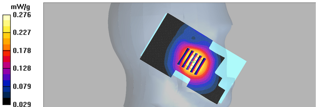
Fig.5 WCDMA 850 CH4233
