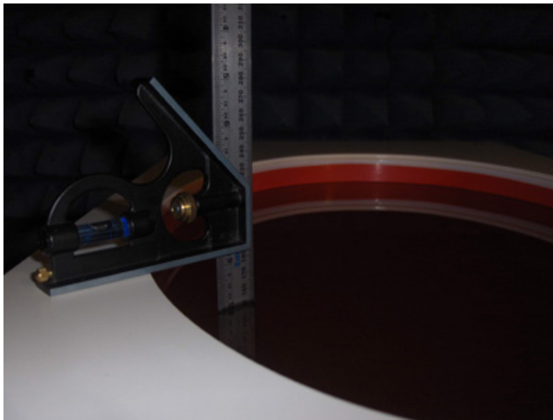
150MHz Tissue Liquid
