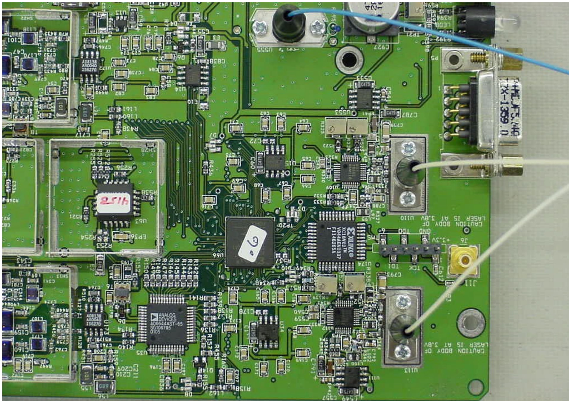
Digivance LRCS 1900 MHz Signal Transport Module Control Board - T3
