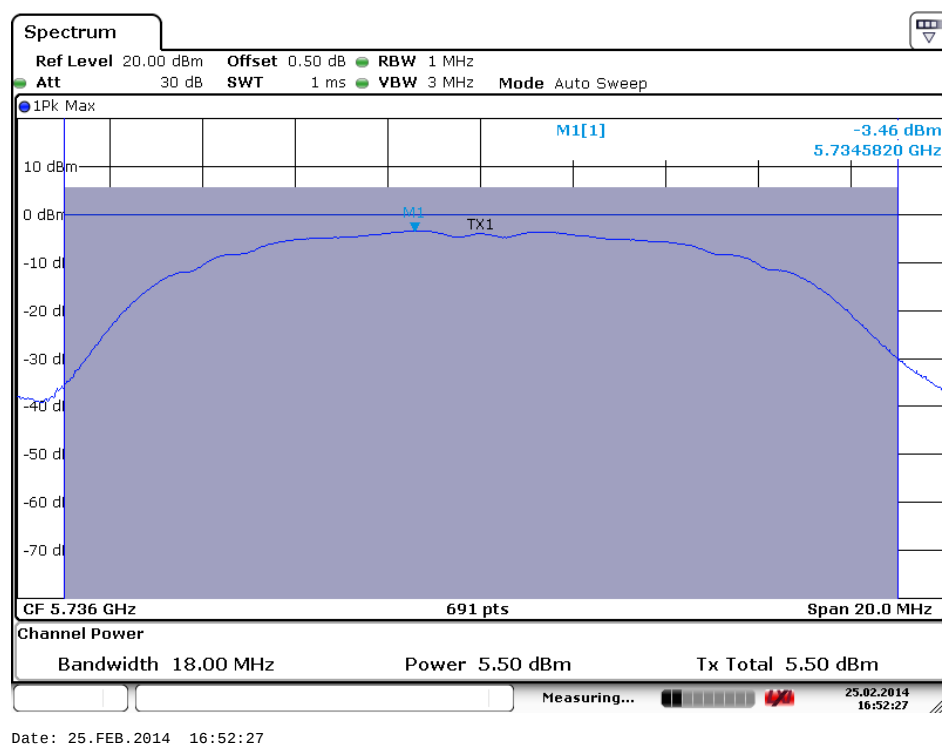
Low channel (Antenna A)
