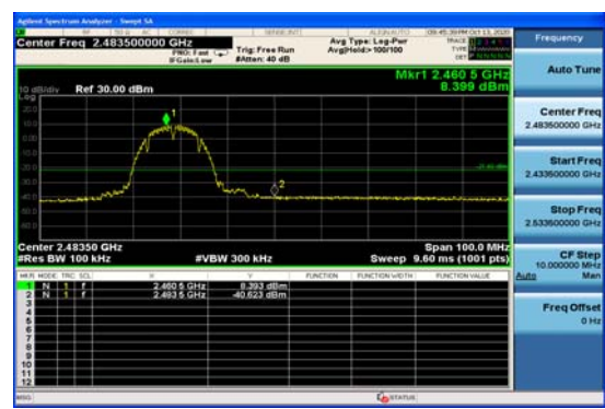
802.11g, Channel No.: 11
