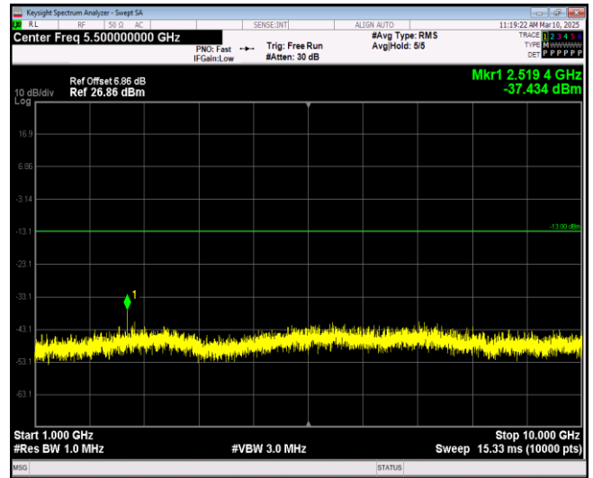
Band5-10MHz-64QAM-20450-1RB#0-Range2:1000~10000MHz
