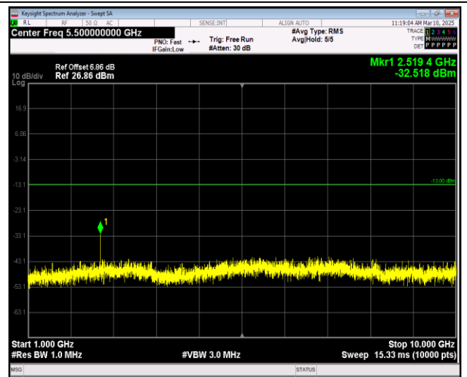
Band5-10MHz-16QAM-20450-1RB#0-Range2:1000~10000MHz
