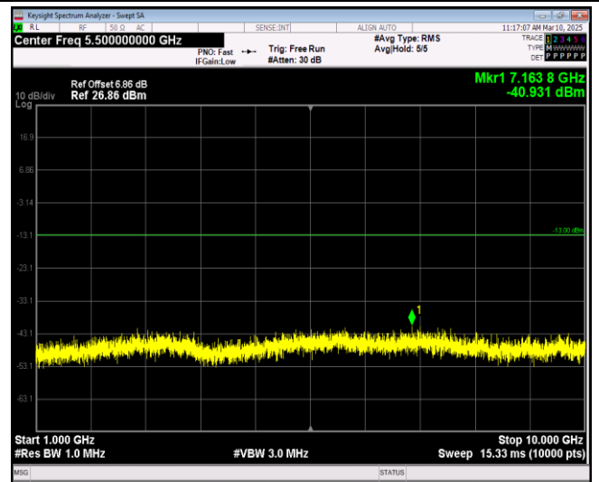
Band5-10MHz-16QAM-20525-1RB#0-Range2:1000~10000MHz
