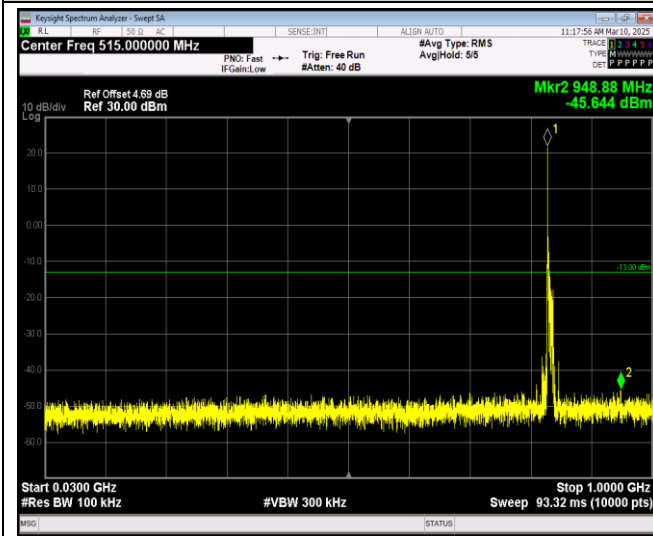
Band5-10MHz-16QAM-20525-1RB#0-Range1:30~1000MHz
