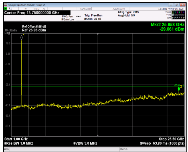
Band7-20MHz-64QAM-21350-1RB#0-Range2:1000~26500MHz
