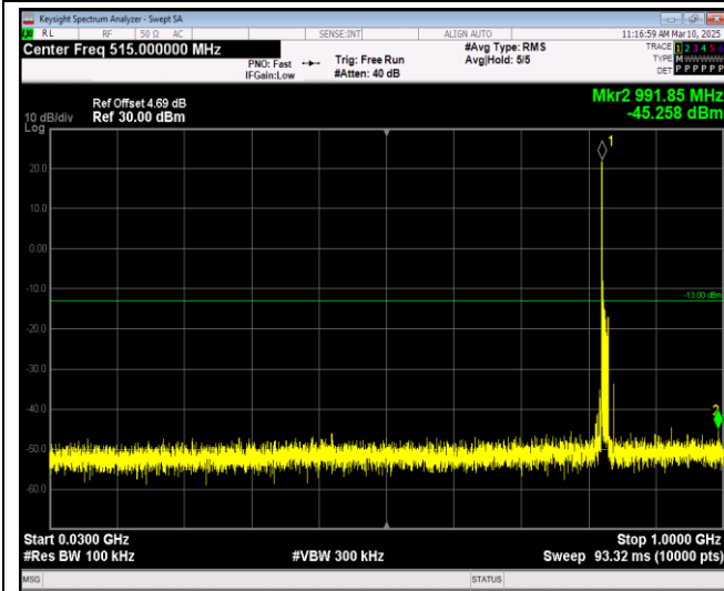
Band5-10MHz-16QAM-20525-1RB#0-Range1:30~1000MHz
