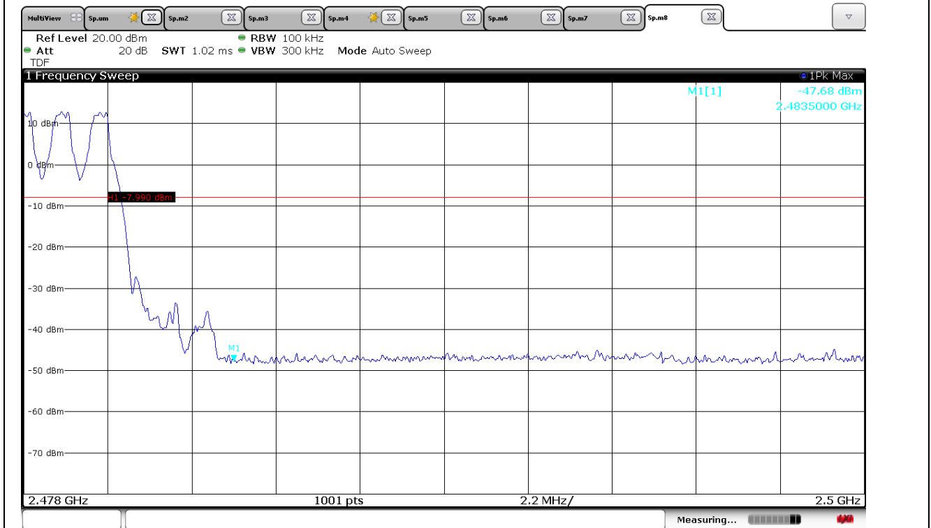
BDR_Hopping_High CH
