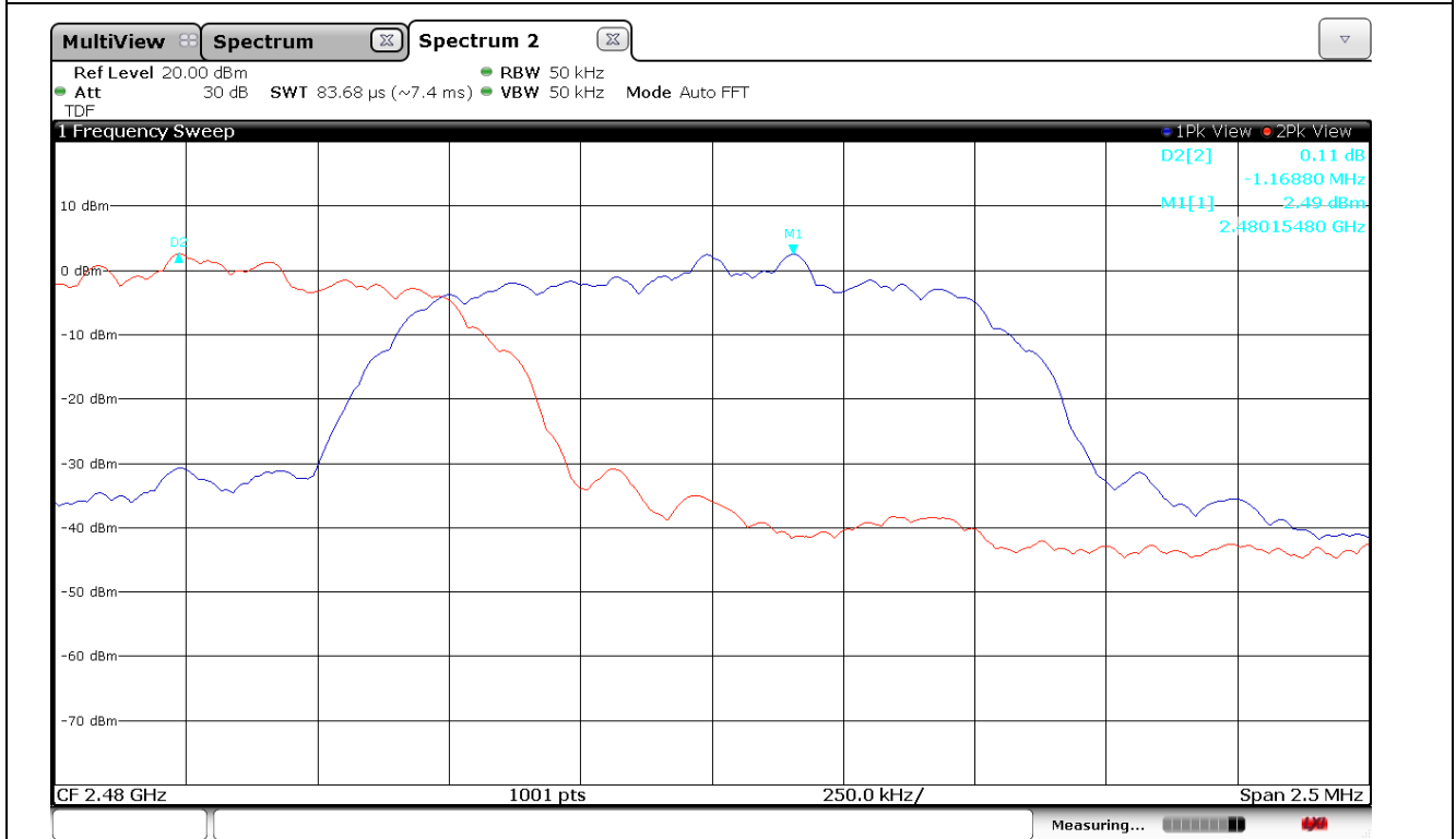
EDR_High CH
