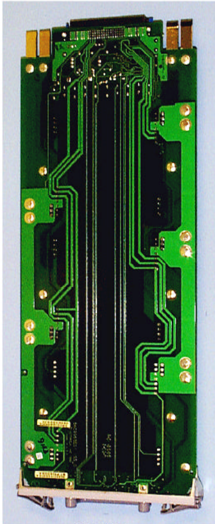
IHET5BL1 SC4812T @ 800MHz Power Supply Back
