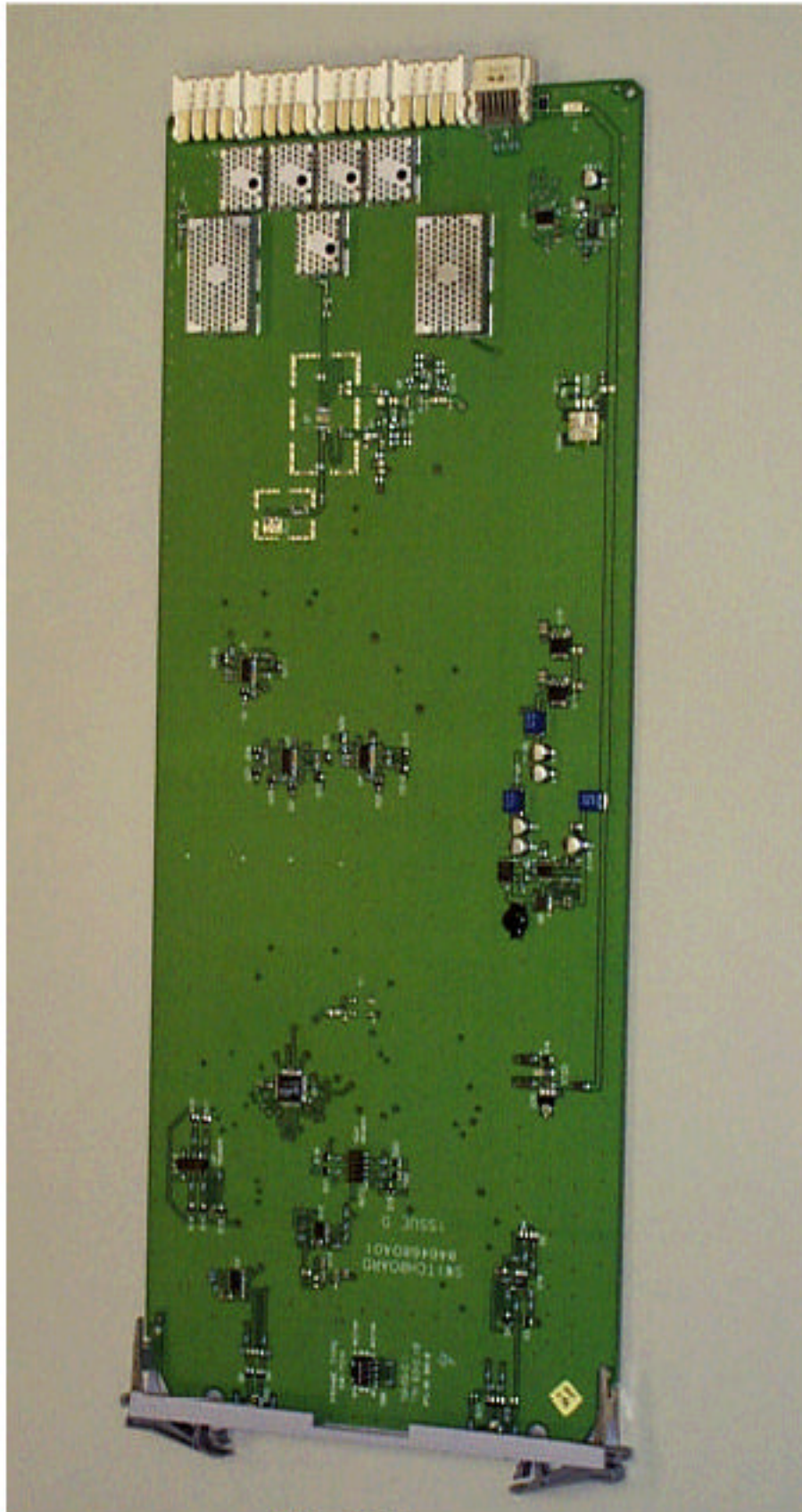
IHET5BL1 SC4812T @ 800MHz Switch Card Front
