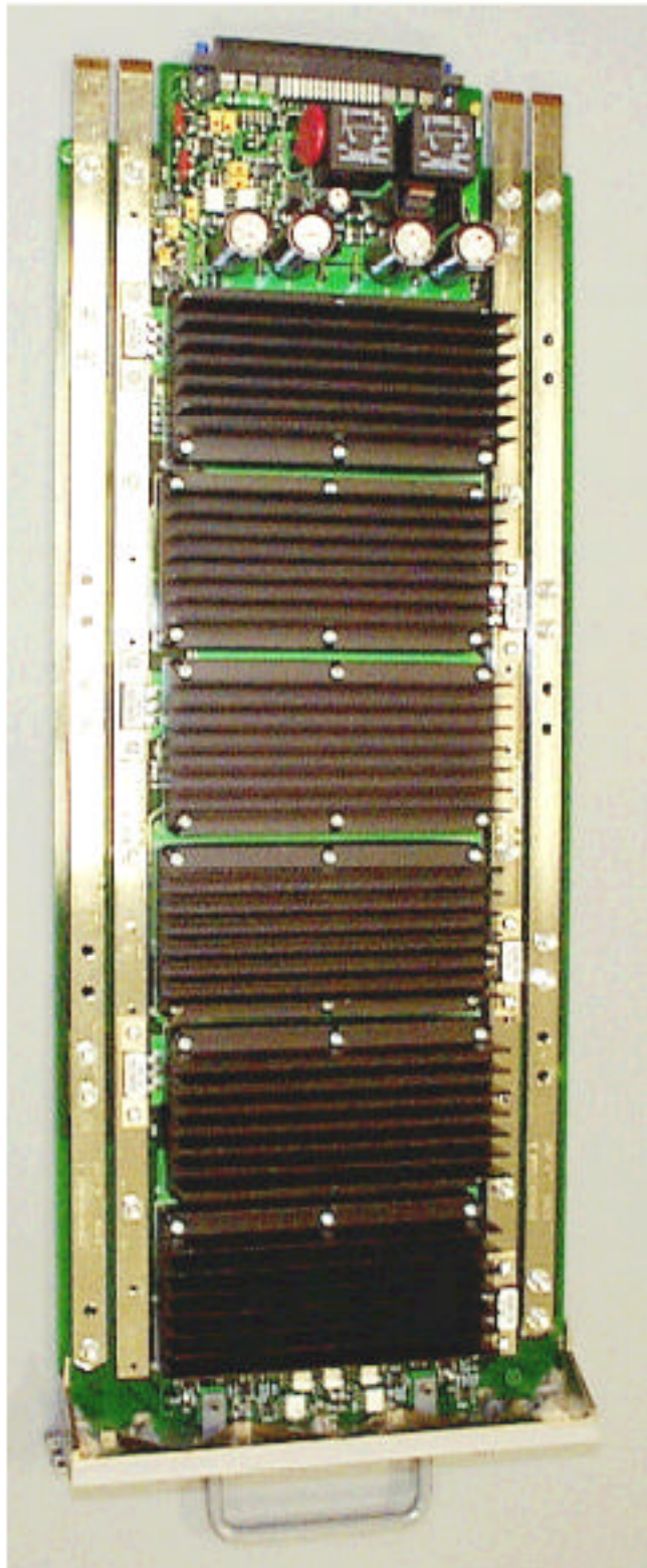
IHET5BL1 SC4812T @ 800MHz Power Supply Front
