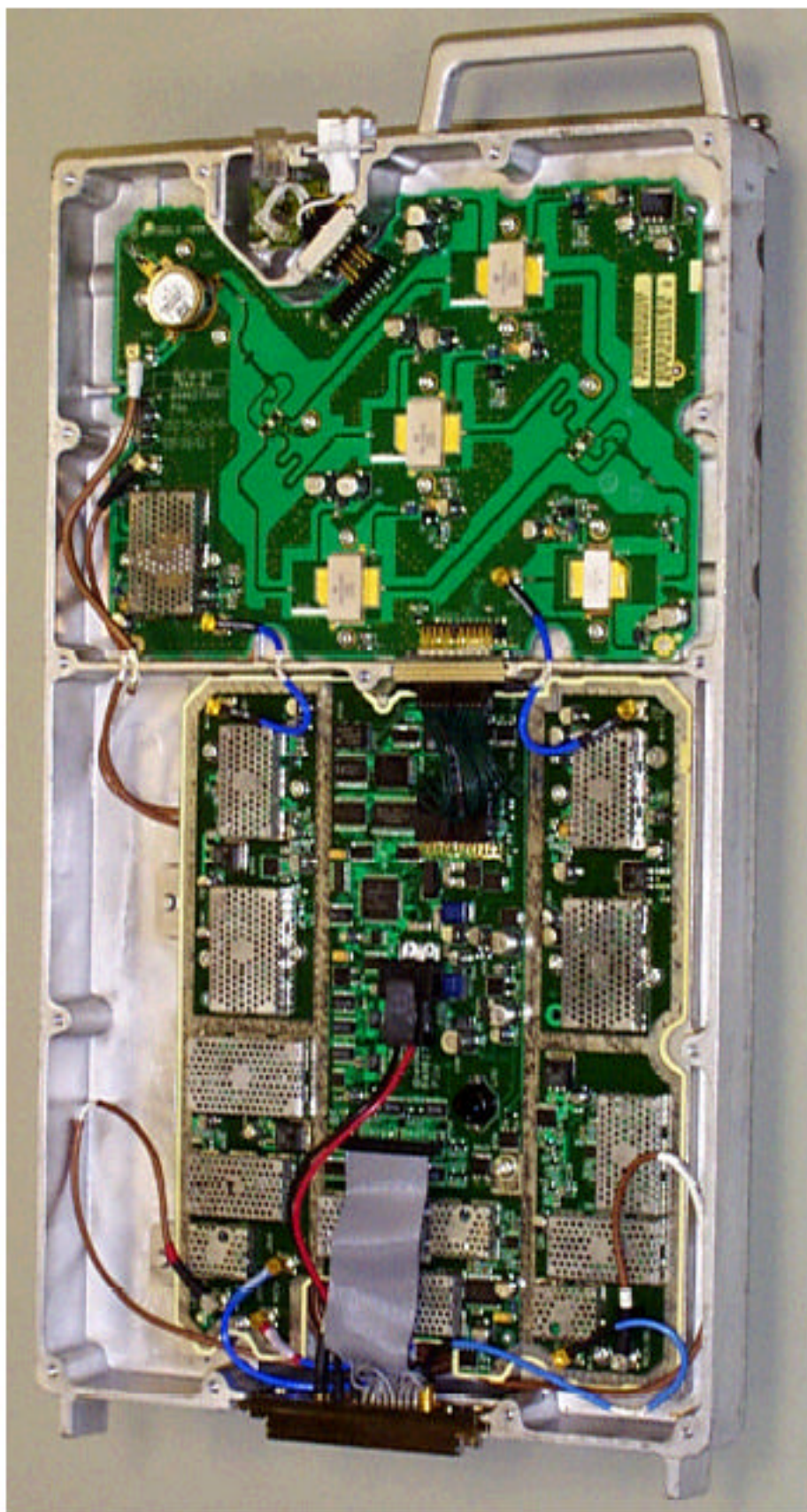
IHET5BL1 SC4812T @ 800MHz LPA without Cover
