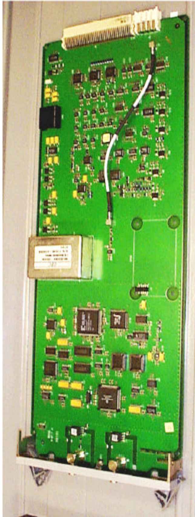
IHET5BL1 SC4812T @ 800MHz CSM2 Front
