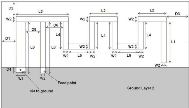
Figure 3: Antenna Dimensions
