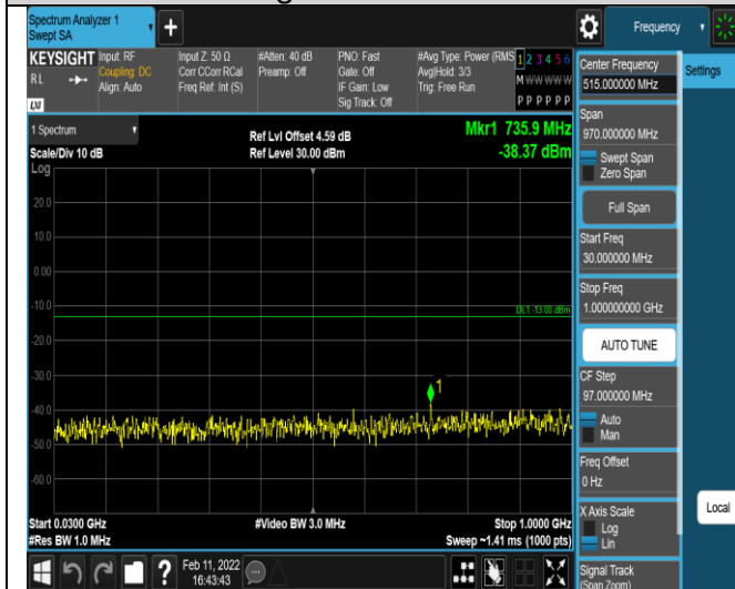
Band2-1.4MHz-QPSK-18900-1RB#0- Range1:30~1000MHz
