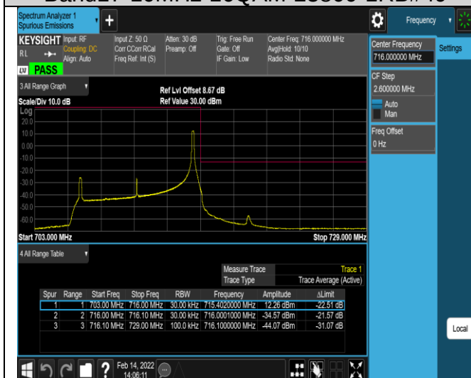
Band17-10MHz-16QAM-23800-1RB#49
