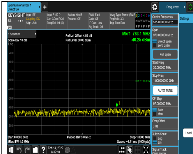
Band2-20MHz-16QAM-19100-1RB#0- Range1:30~1000MHz
