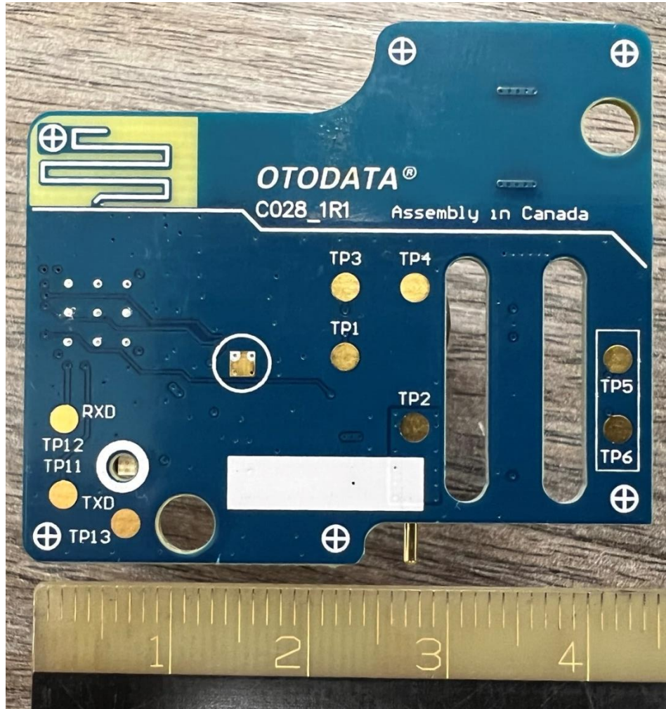
Figure 2: PCB bottom view
