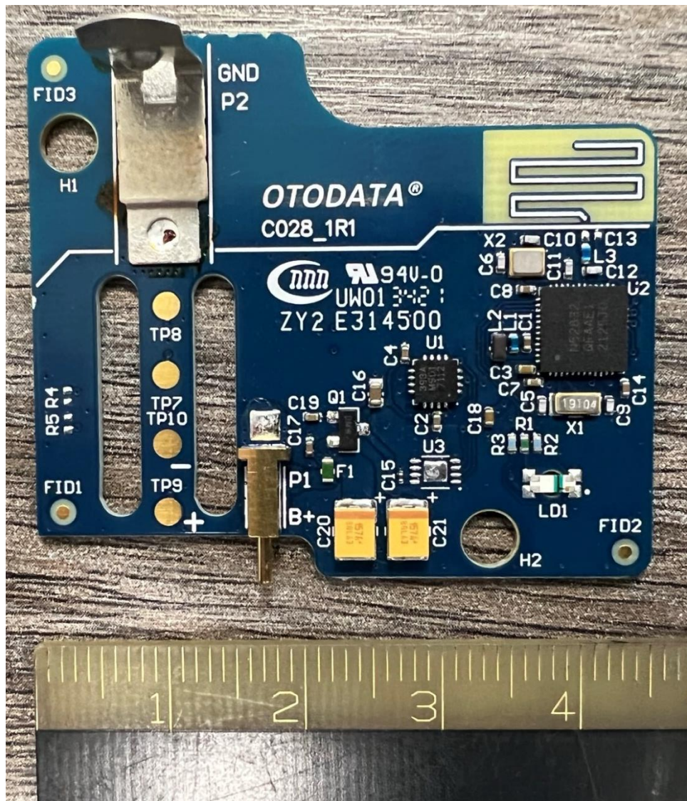
Figure 3: PCB top view
