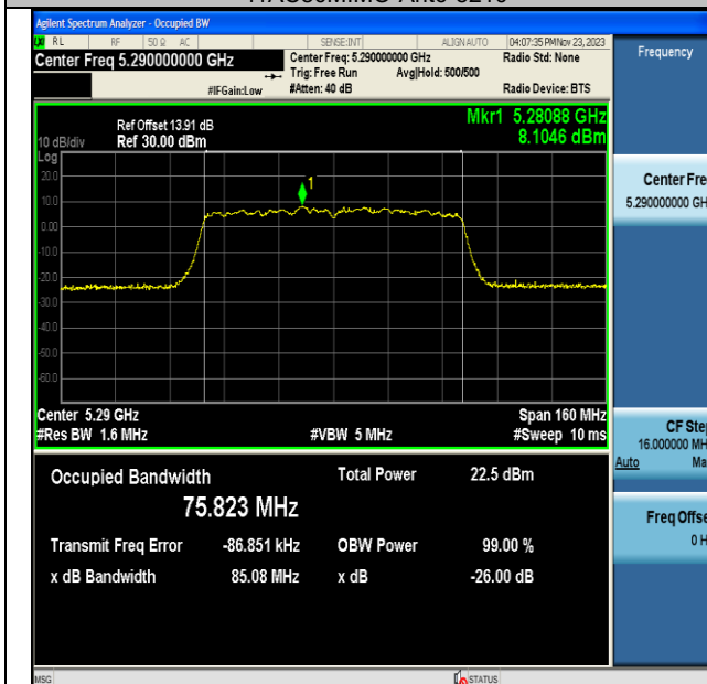
11AC80MIMO-Ant6-5290
