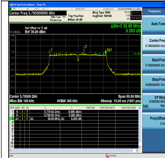
11AC40MIMO-Ant6-5795-PASS
