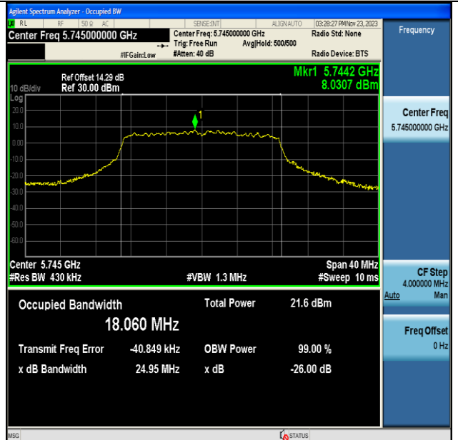
11AC20MIMO-Ant7-5745
