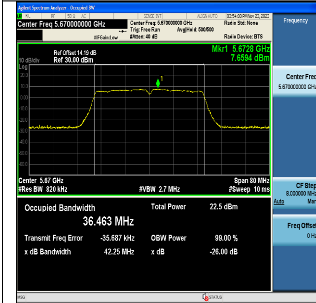
11AC40MIMO-Ant6-5670
