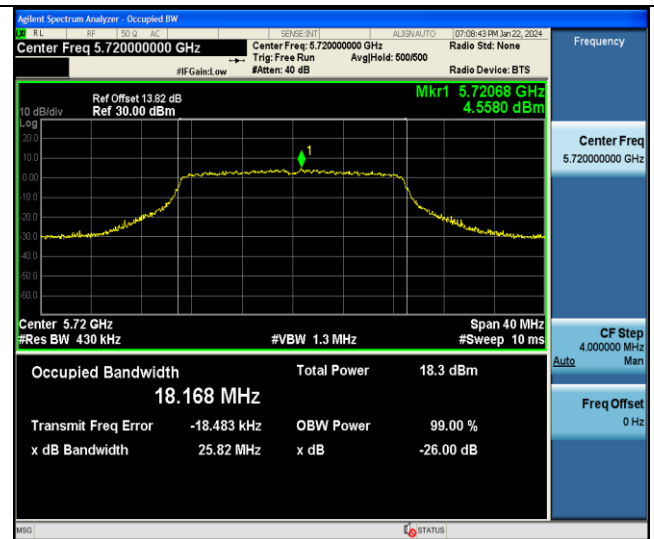
11AC20MIMO-Ant7-5720
