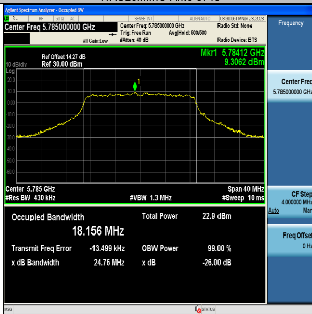
11AC20MIMO-Ant6-5785
