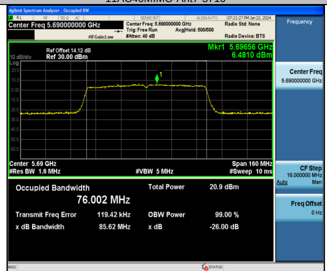
11AC80MIMO-Ant7-5690
