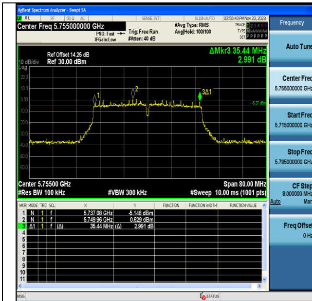
11AC40MIMO-Ant6-5755-PASS
