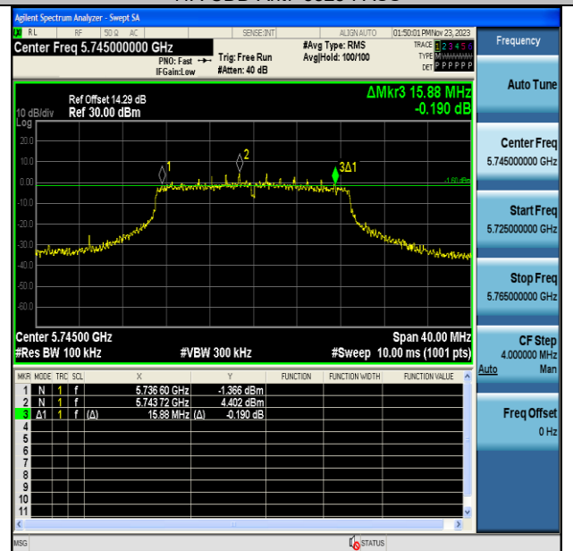
11N20MIMO-Ant7-5745-PASS
