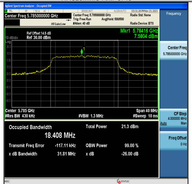
11AC20MIMO-Ant7-5785
