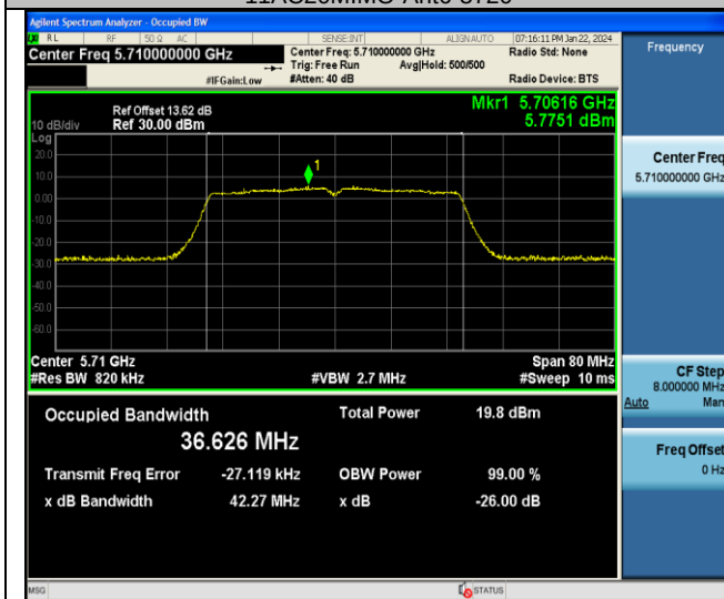
11AC40MIMO-Ant6-5710
