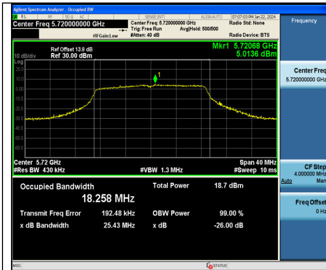
11AC20MIMO-Ant6-5720
