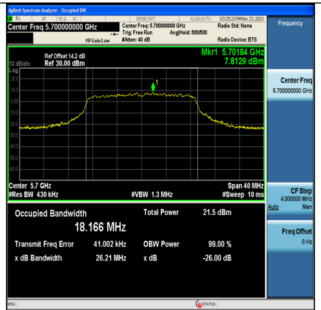
11AC20MIMO-Ant7-5700
