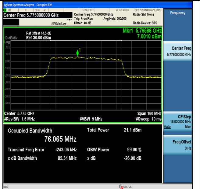
11AC80MIMO-Ant7-5775
