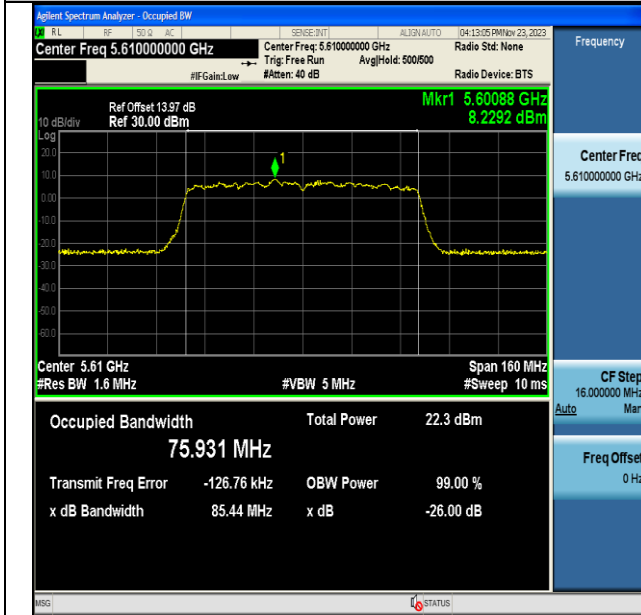
11AC80MIMO-Ant6-5610
