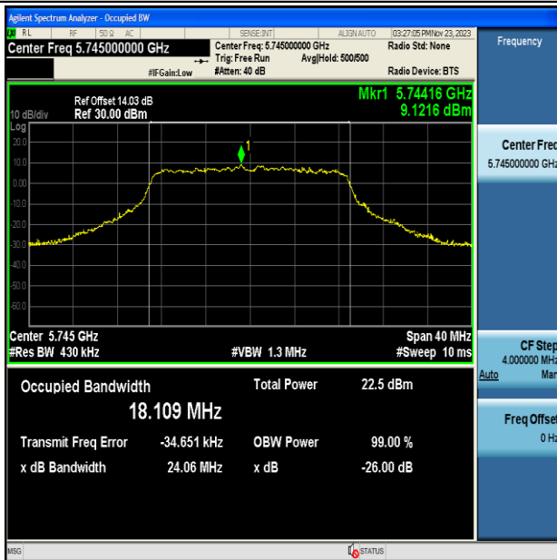
11AC20MIMO-Ant6-5745
