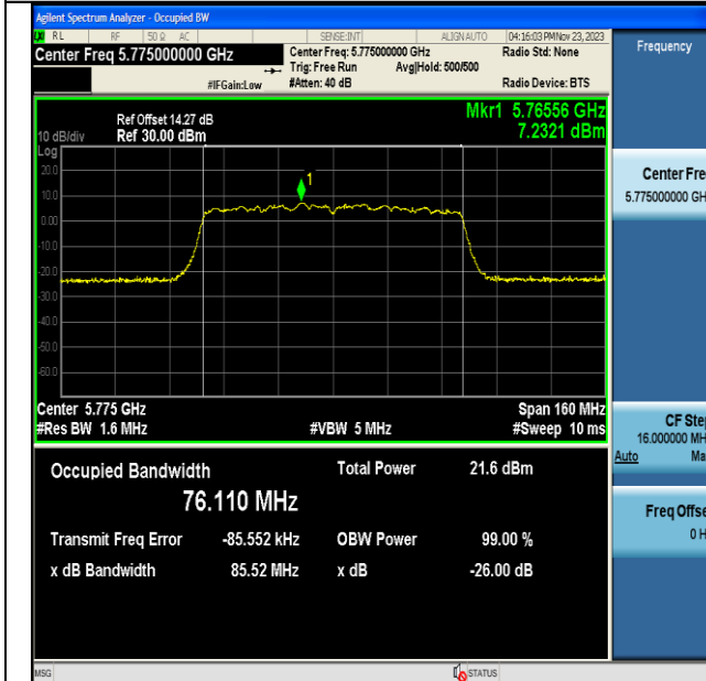
11AC80MIMO-Ant6-5775
