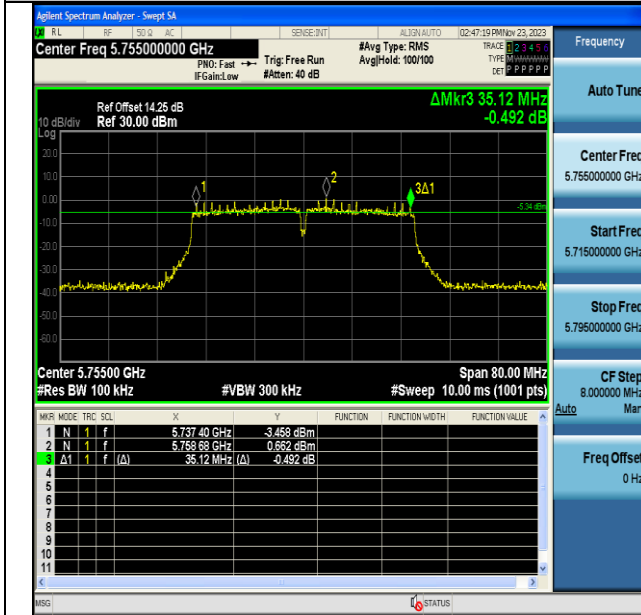
11N40MIMO-Ant6-5755-PASS
