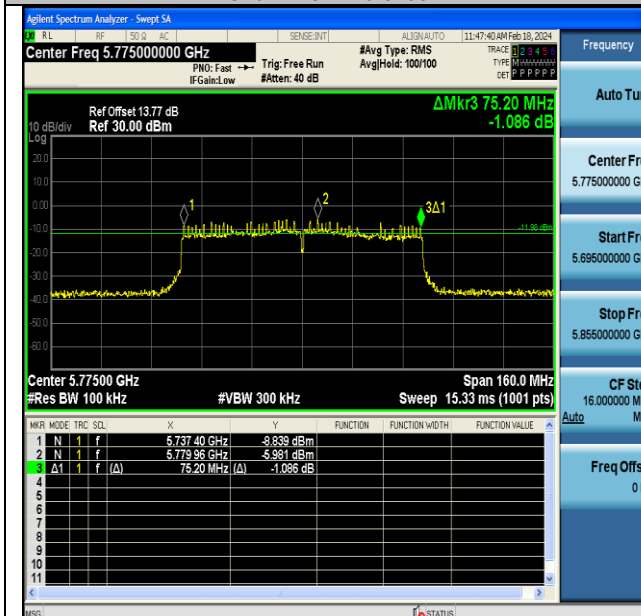
11AC80MIMO-Ant6-5775-PASS
