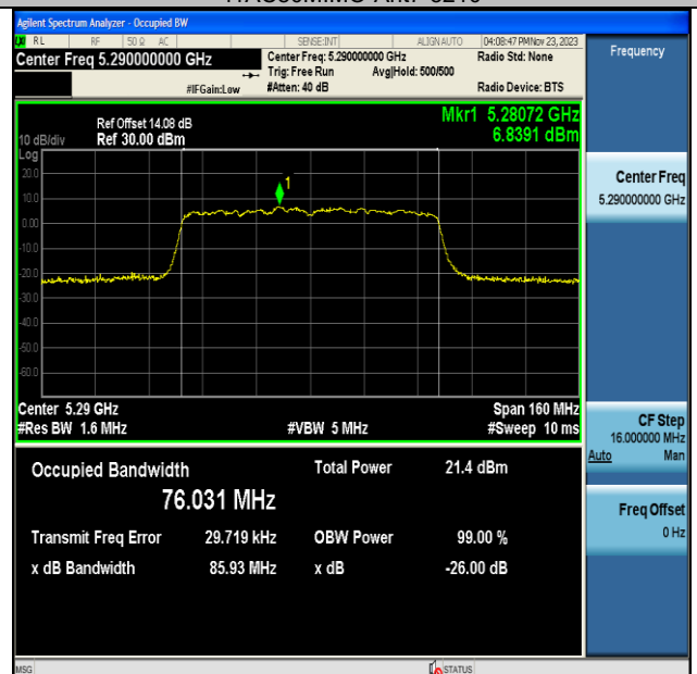
11AC80MIMO-Ant7-5290
