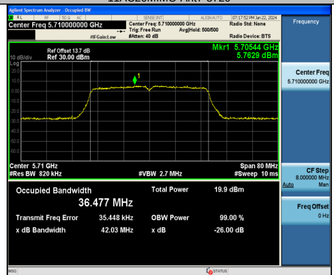
11AC40MIMO-Ant7-5710
