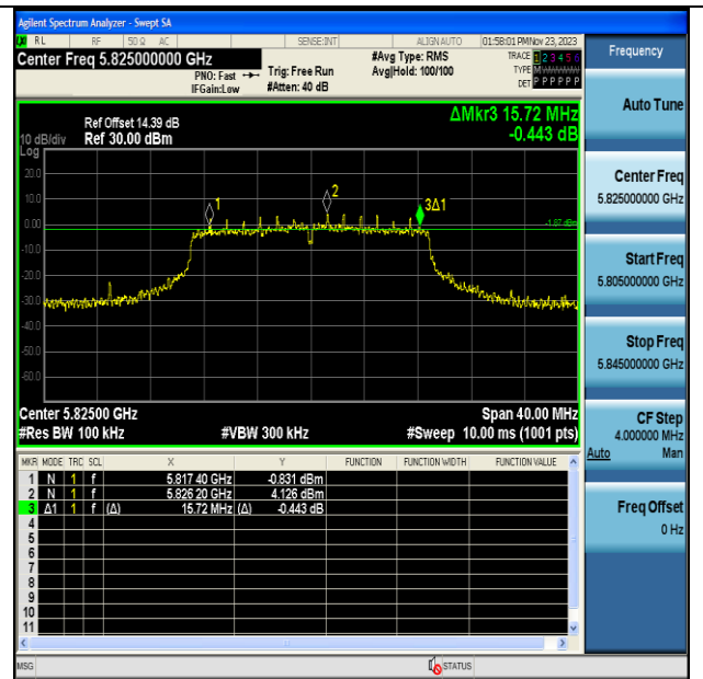
11N20MIMO-Ant7-5825-PASS
