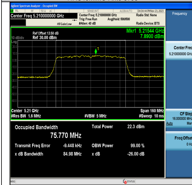
11AC80MIMO-Ant6-5210
