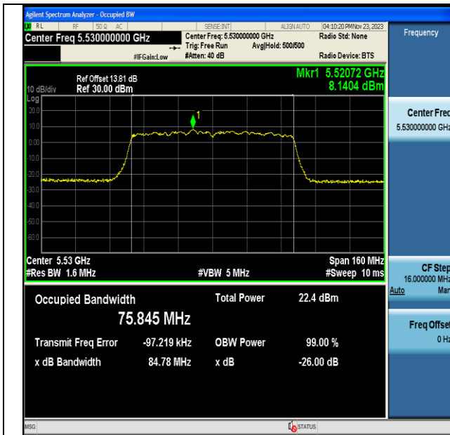
11AC80MIMO-Ant6-5530
