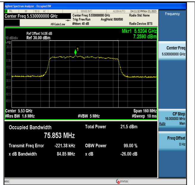
11AC80MIMO-Ant7-5530
