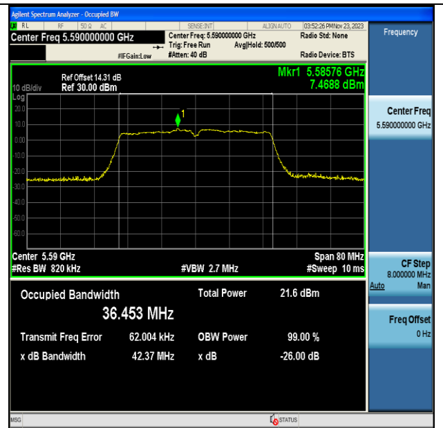
11AC40MIMO-Ant7-5590
