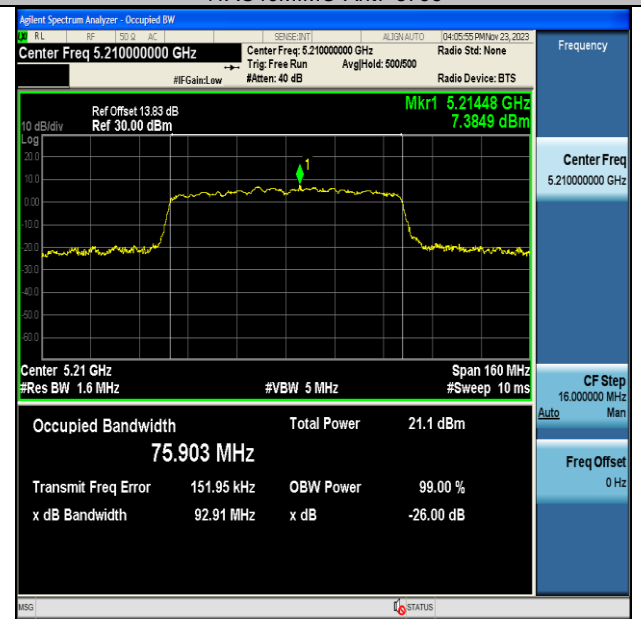
11AC80MIMO-Ant7-5210
