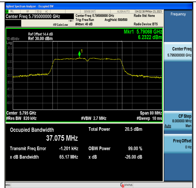
11AC40MIMO-Ant7-5795
