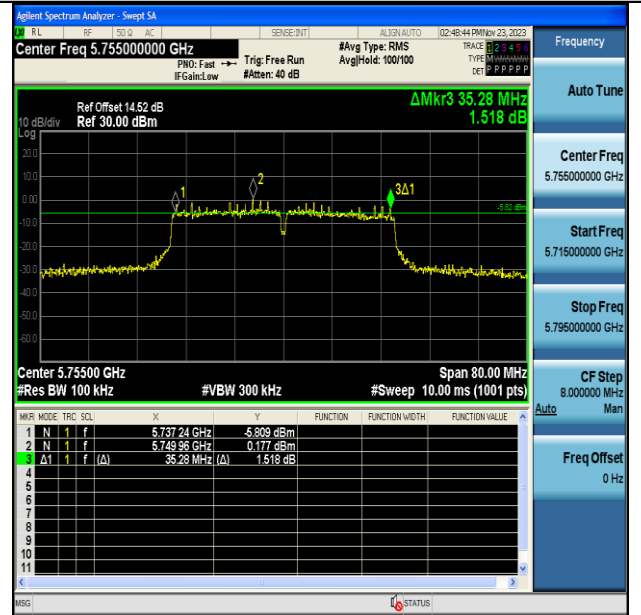
11N40MIMO-Ant7-5755-PASS
