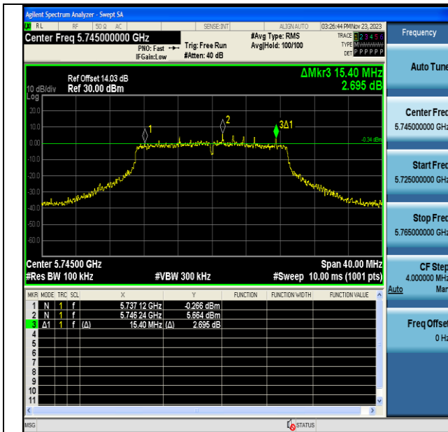
11AC20MIMO-Ant6-5745-PASS
