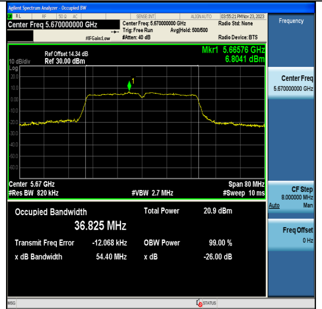
11AC40MIMO-Ant7-5670
