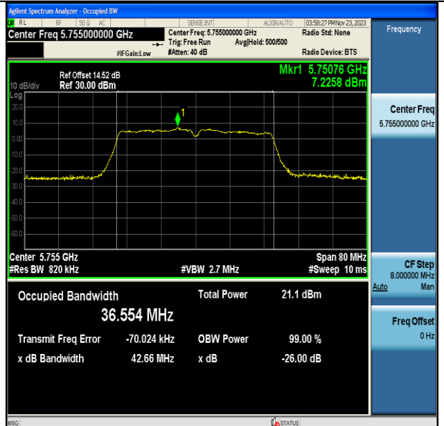
11AC40MIMO-Ant7-5755
