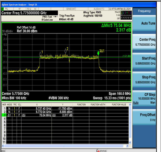
11AC80MIMO-Ant7-5775-PASS
