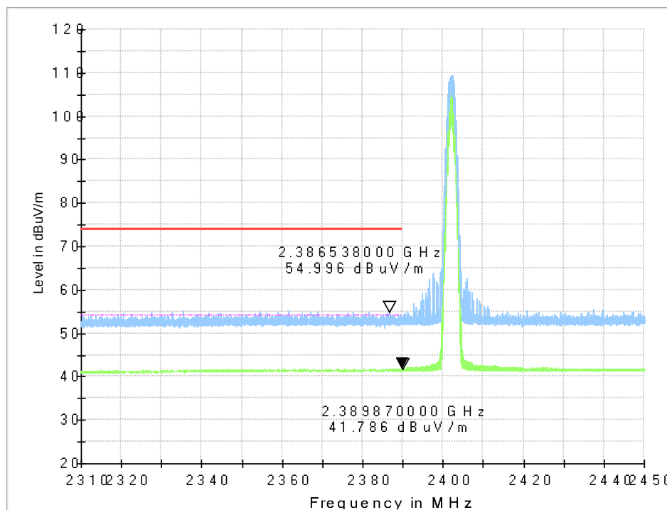
Fig.13. Frequency Band Edges: GFSK, Channel 0, Hopping Off, 2.31 GHz – 2.45GHz
