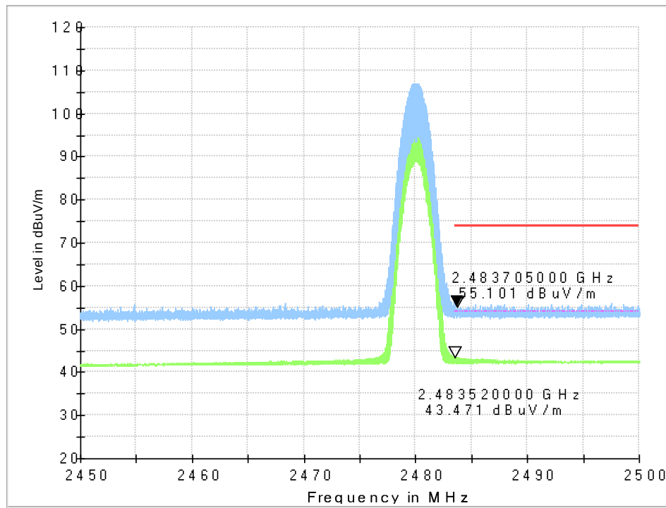
Fig.18. Frequency Band Edges: 8DPSK, Channel 78, 2.45 GHz - 2.50GHz
