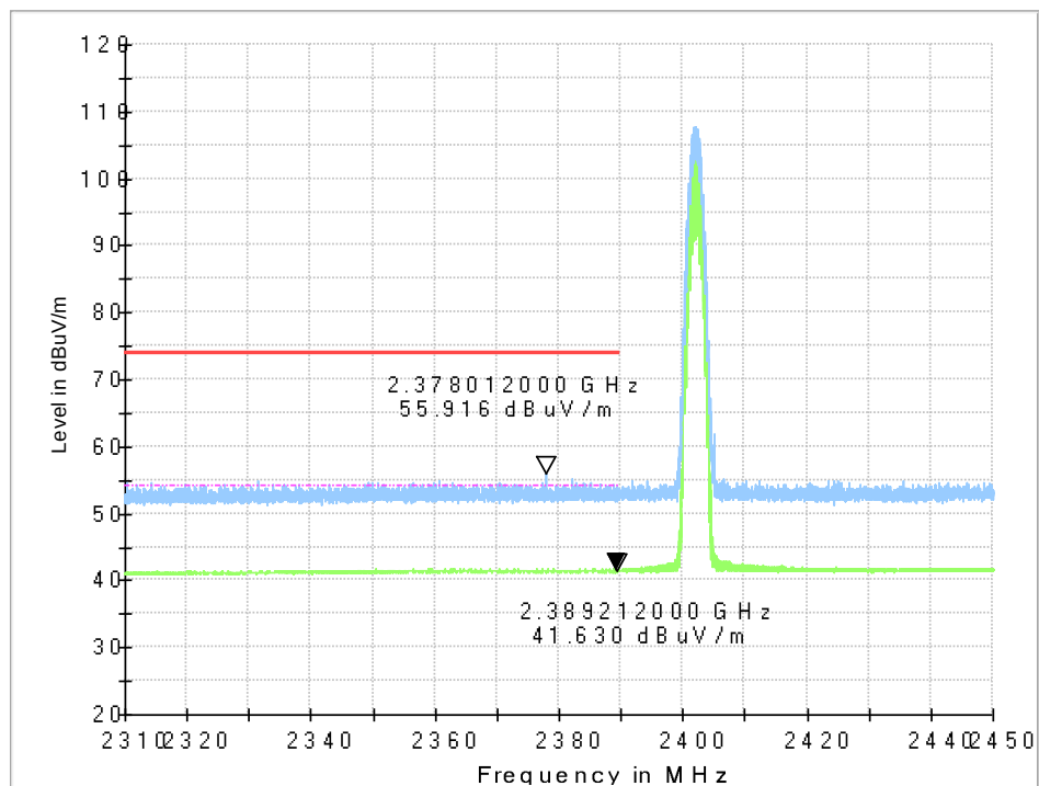
Fig.17. Frequency Band Edges: 8DPSK, Channel 0, 2.31 GHz - 2.45GHz
