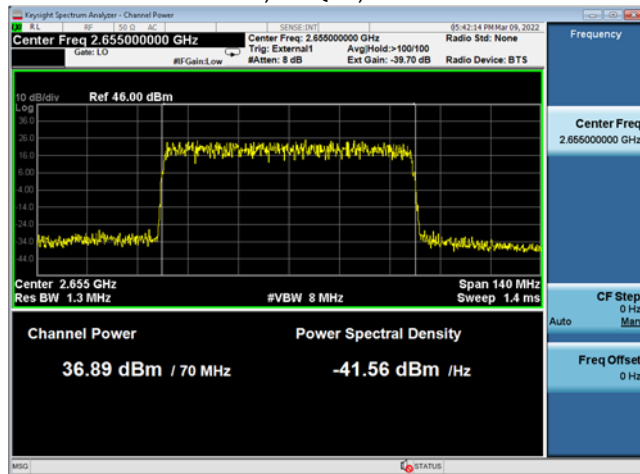
TM3.1a, 256QAM, 2655MHz
