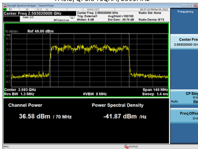
TM3.2, QPSK/16QAM, 2593MHz
