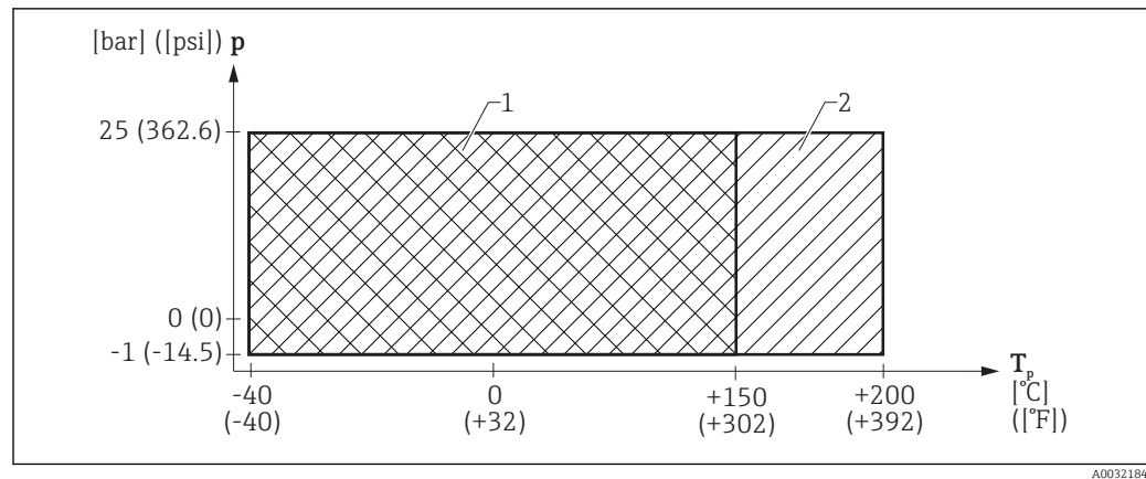
14 FMR62: Permitted range for process temperature and process pressure, flange or DIN11851 process connection
