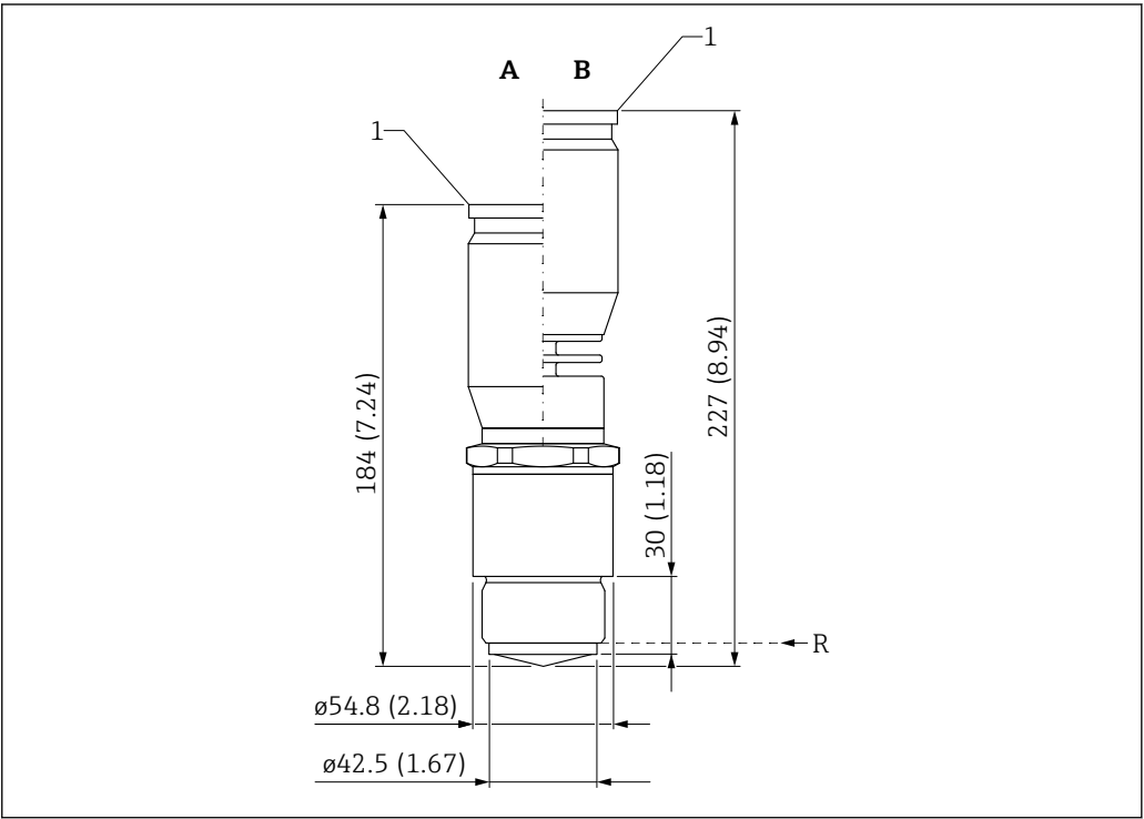
19 Dimensions: mm (in)
