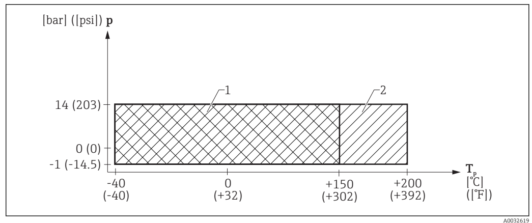
13 FMR62: Permitted range for process temperature and process pressure, Tri-Clamp 3" or Tri-Clamp 4" process connection
