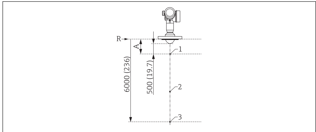
29 Points of the 3-point linearity protocol; engineering unit: mm (in)
