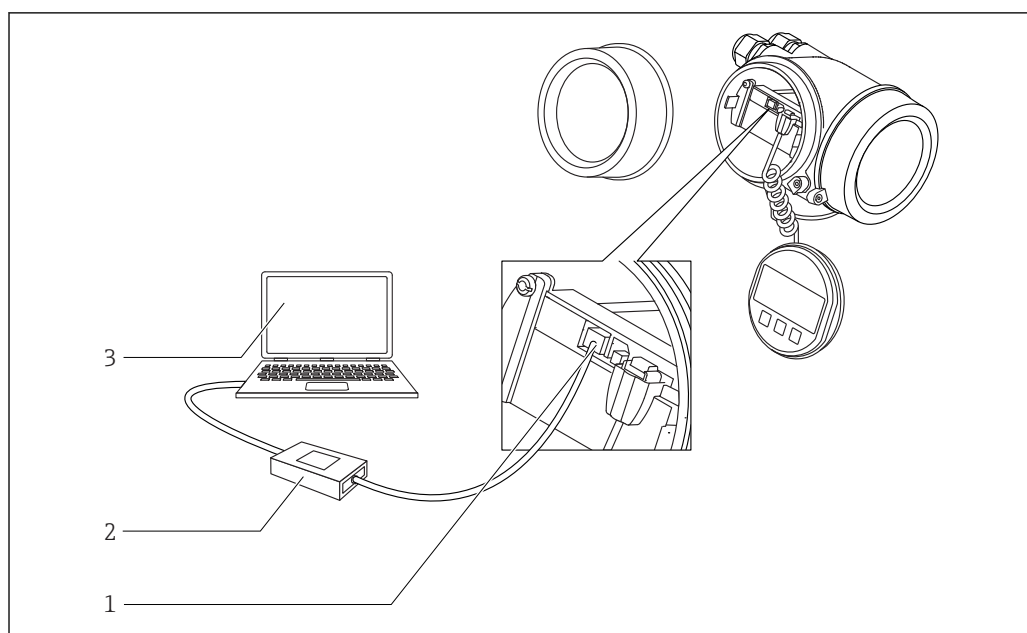
26 DeviceCare/FieldCare via service interface (CDI)
