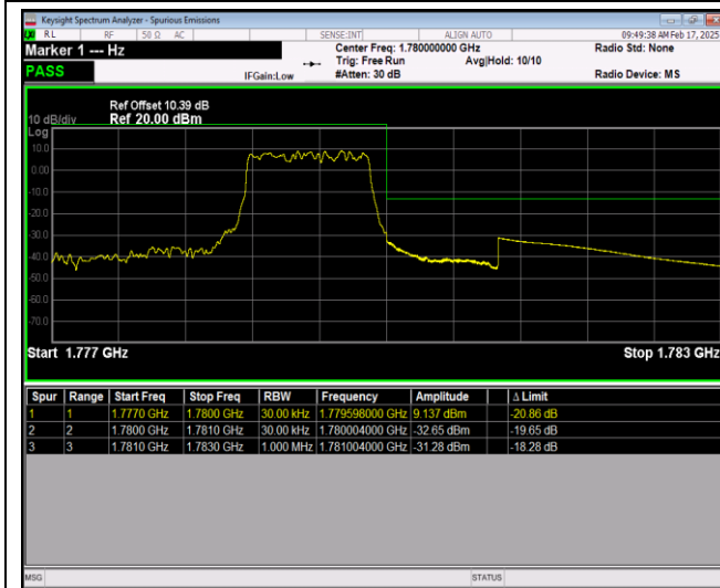
Band66-1.4MHz-16QAM-131979-1RB#5
