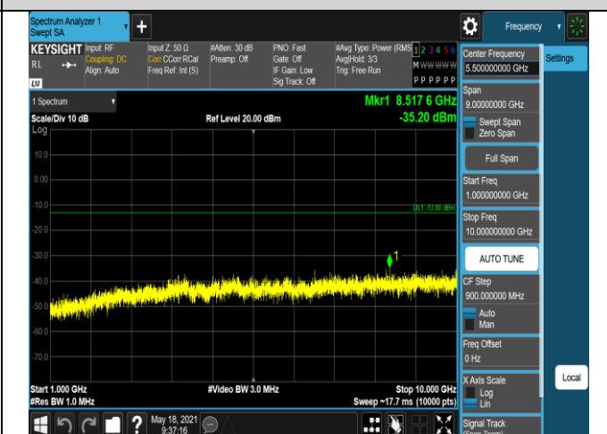
Band5-10MHz-QPSK-20525-1RB#0-Range2:1000~100
