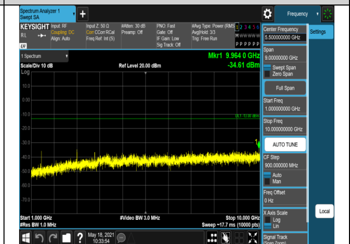
Band12-10MHz-QPSK-23095-1RB#0-Range2:1000~10
