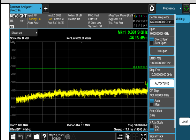
Band5-10MHz-QPSK-20600-1RB#0-Range2:1000~100
