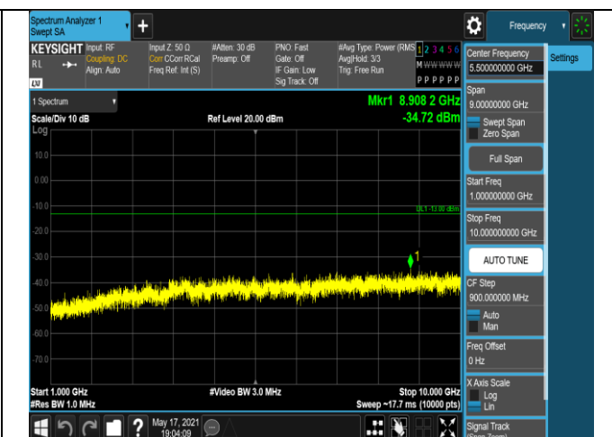
Band5-10MHz-QPSK-20450-1RB#0-Range2:1000~100
