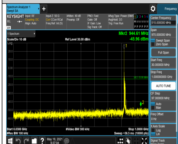
Band5-10MHz-QPSK-20525-1RB#0-Range1:30~10
