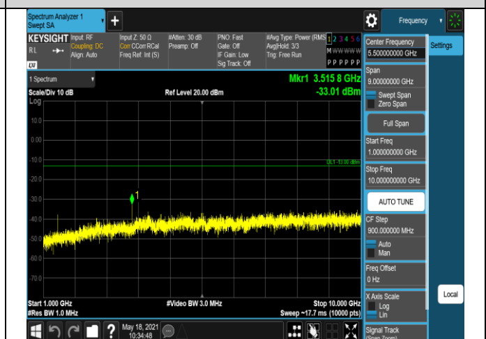
Band12-10MHz-QPSK-23130-1RB#0-Range2:1000~10
