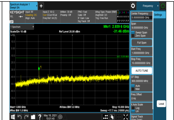
Band12-10MHz-QPSK-23060-1RB#0-Range2:1000~10
