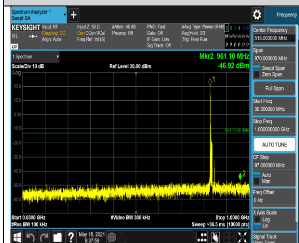
Band5-10MHz-QPSK-20600-1RB#0-Range1:30~10
