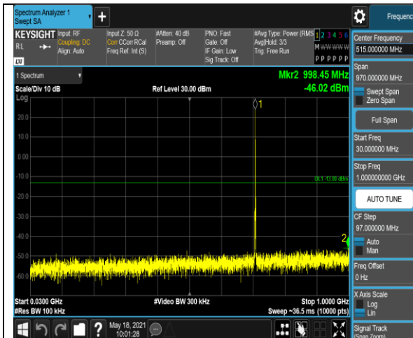
Band12-10MHz-QPSK-23060-1RB#0-Range1:30~1
