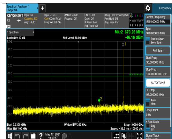
Band5-10MHz-QPSK-20450-1RB#0-Range1:30~10
