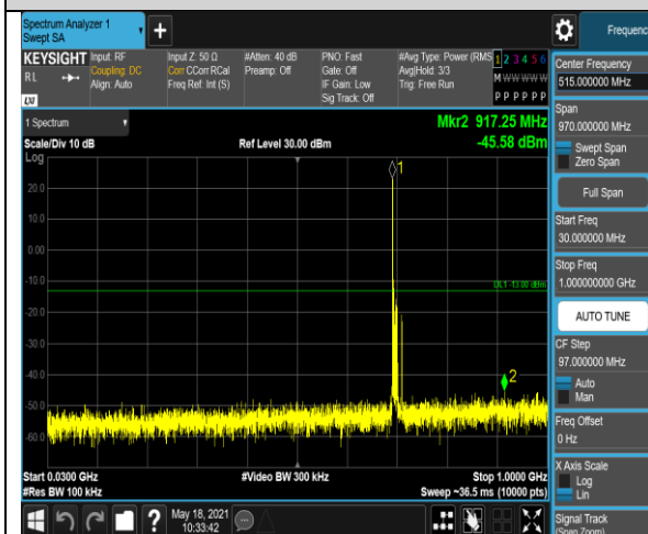
Band12-10MHz-QPSK-23095-1RB#0-Range1:30~1
