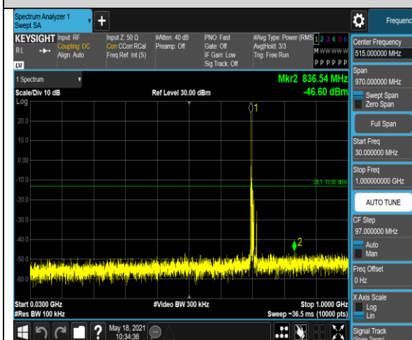
Band12-10MHz-QPSK-23130-1RB#0-Range1:30~1
