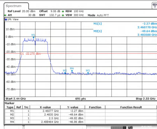
11G-Ant1-2462-PASS
