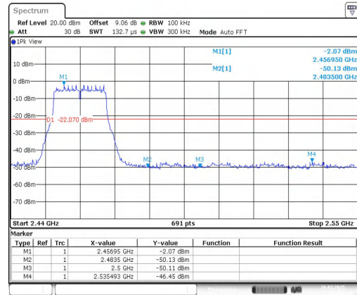
11B-Ant1-2462-PASS
