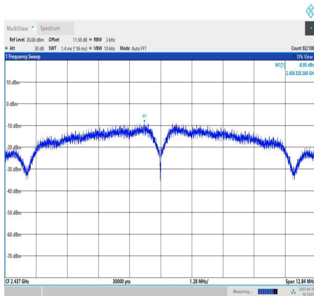
11B-Ant1-2437-PASS
