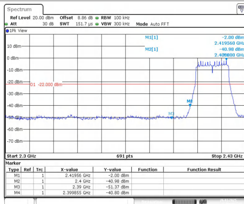
11G-Ant1-2412-PASS
