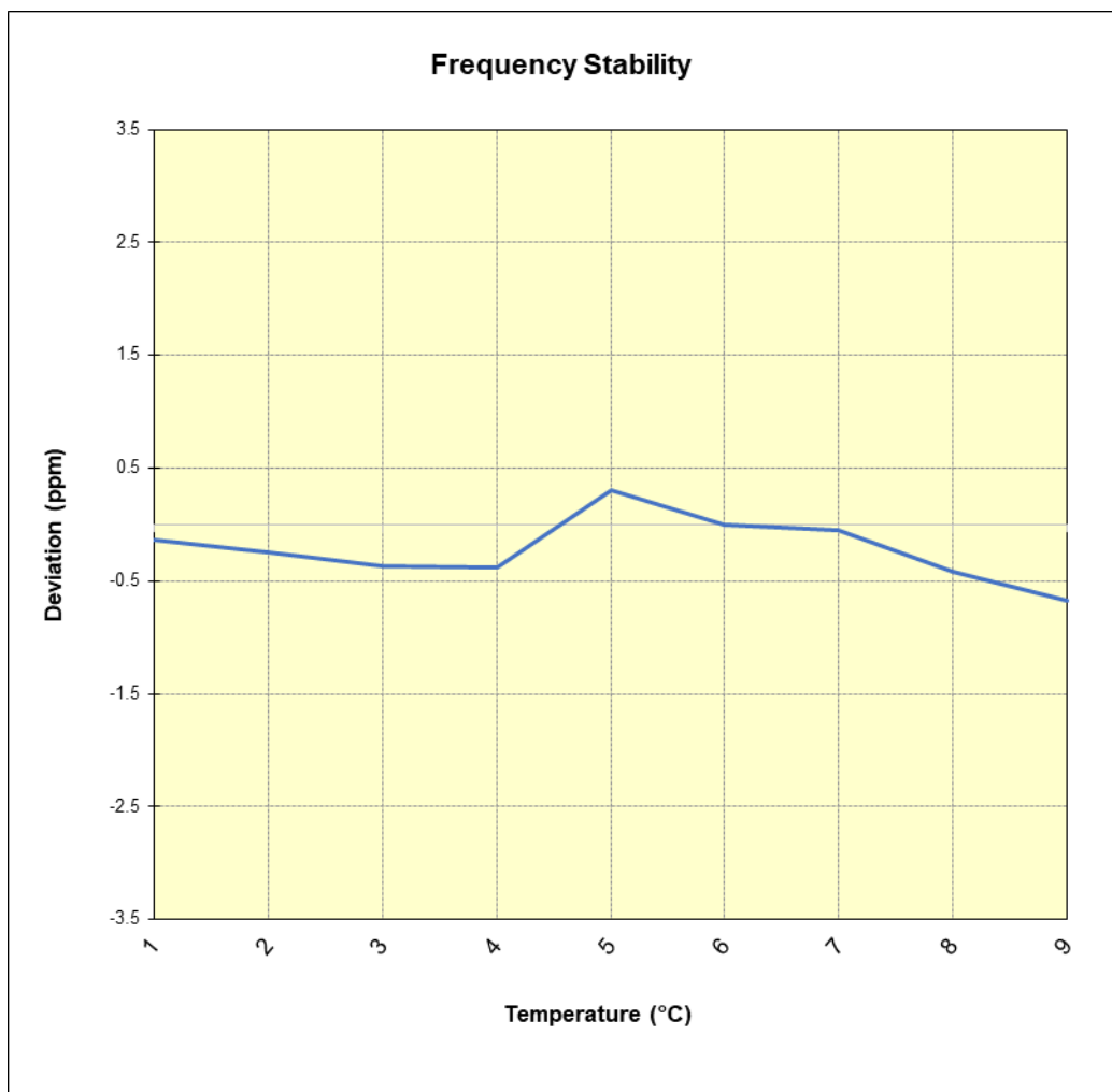
Plot 7-37. LTE Band 8 NB-IoT Frequency Stability Chart
