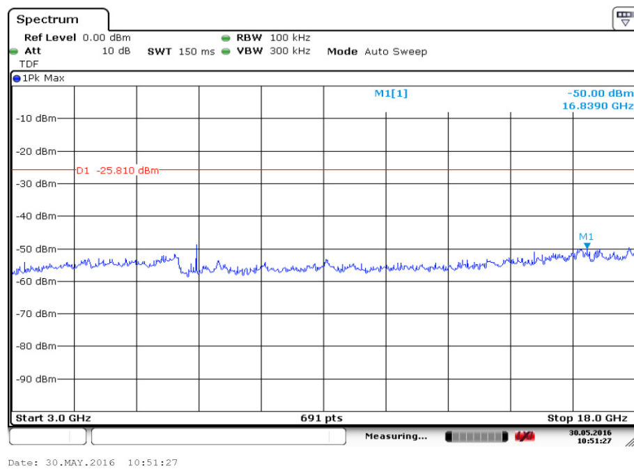
Fig.11. Conducted Spurious Emission (Ch39, 3 GHz-18 GHz)
