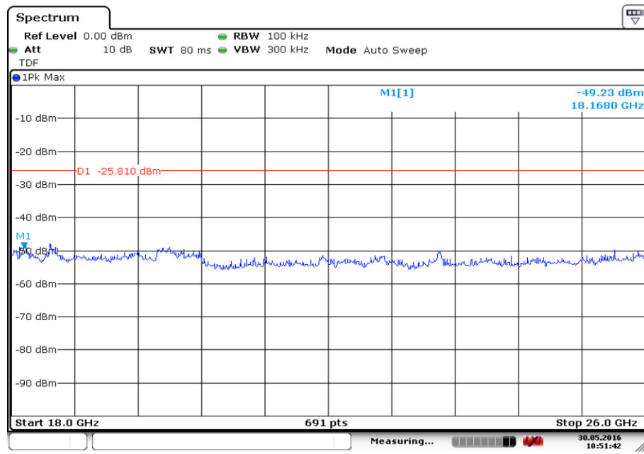
Fig.12. Conducted Spurious Emission (All channels, 18 GHz-26 GHz)
