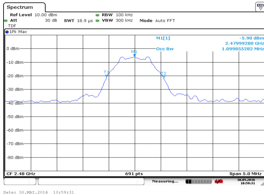
Fig.29. Occupied Bandwidth: GFSK, 2480 MHz
