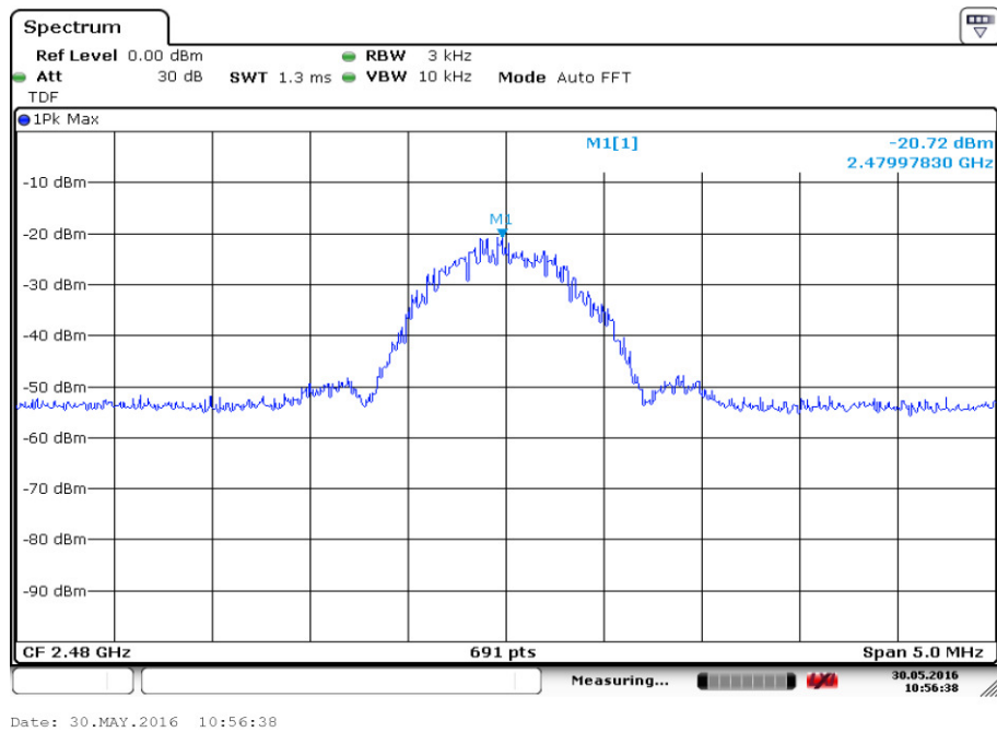
Fig.26. Maximum Power Spectral Density Level Function: GFSK, 2480 MHz
