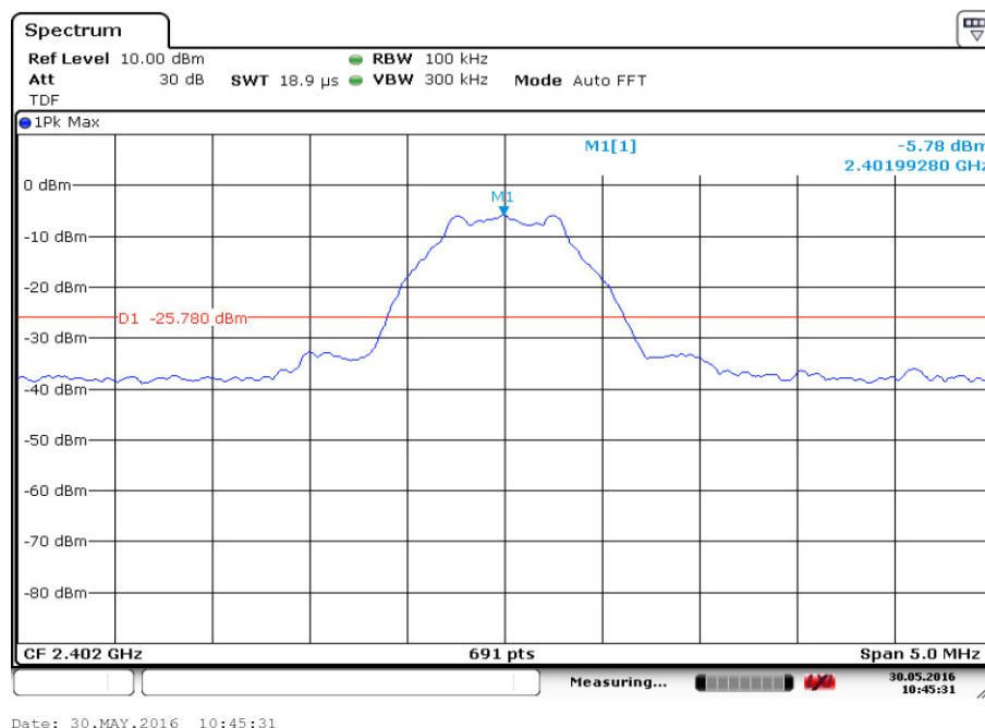
Fig.3. Conducted Spurious Emission (Ch0, Center Frequency)
