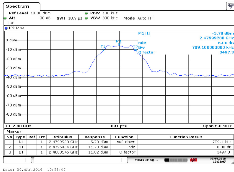
Fig.23. 6dB Bandwidth: GFSK, 2480 MHz
