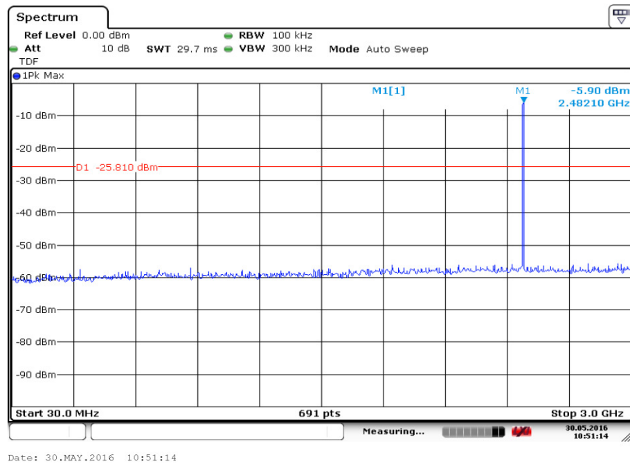
Fig.10. Conducted Spurious Emission (Ch39, 30 MHz-3 GHz)
