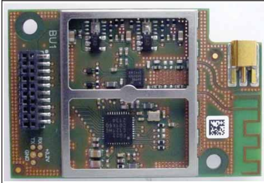
TC242C01_EUT7.2 – conducted sample without shielding
