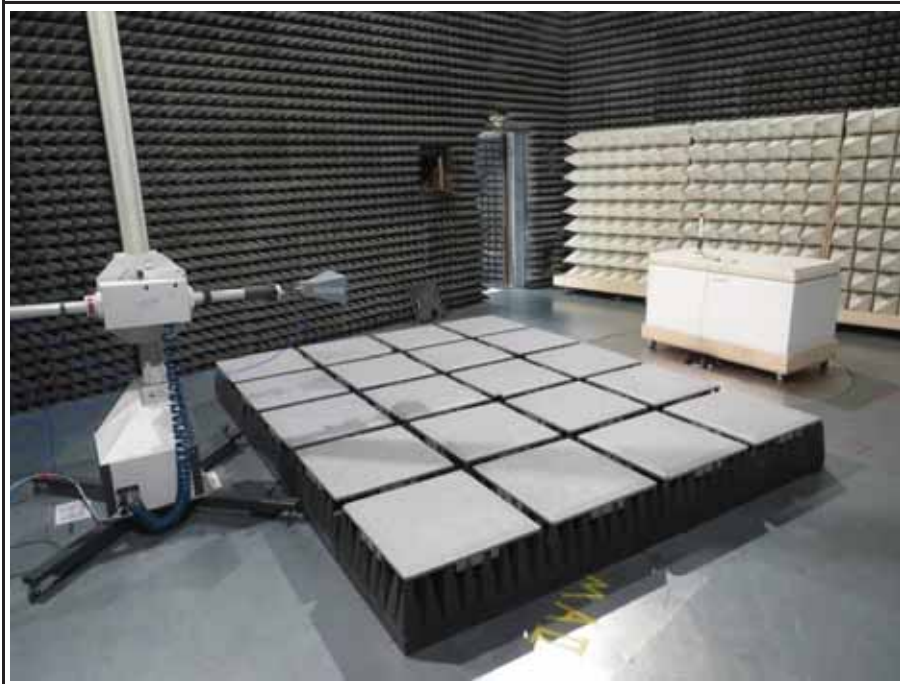
Setup for measurements above 1 GHz (2)
