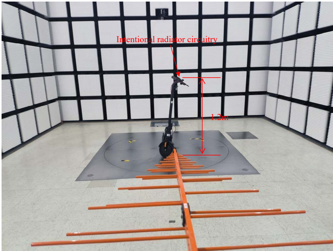
Radiated Emission Below 1GHz View - SPU:V40 Pro
