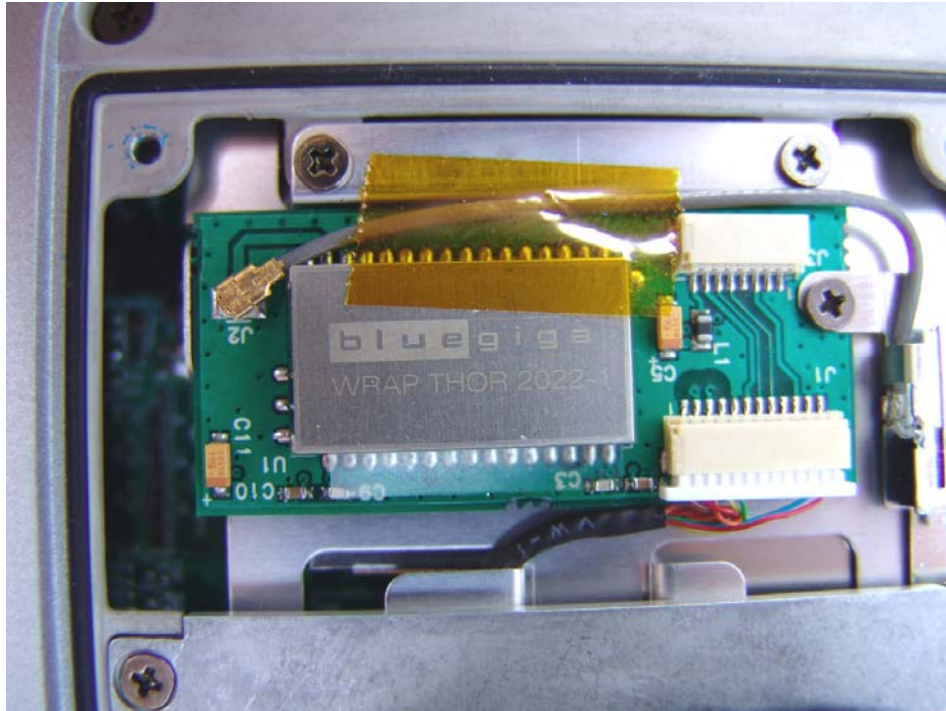
BT2022 removed to show antenna PIFA antenna
